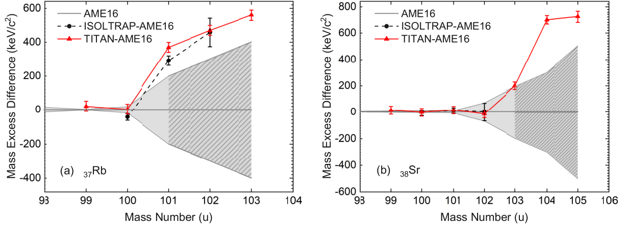
FIG. 2. Mass excess difference between the value measured in this work and the value reported in AME2016 [16], i.e., \text{ME}_{\text{TITAN}} - \text{ME}_{\text{AME2016}} for (a) ^{37}\text{Rb} and (b) ^{38}\text{Sr} isotopes. The shaded band indicates the AME2016 uncertainties, and slanted lines in the shaded region denote values from extrapolation. ME difference is also plotted for a previous measurement from ISOLTRAP [30], published after the AME2016.
