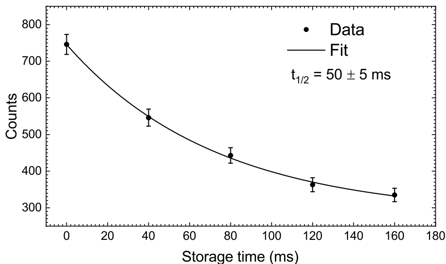
Figure 3. Number of Rb ions recorded as a function of storage time. The error bars on data correspond to statistical error. Solid line represents the exponential fit to data. Half-life obtained from fit agrees with previous value [18, 19].
