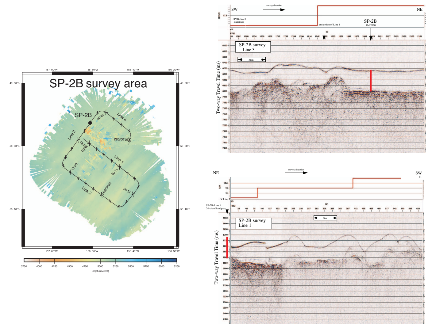
Figure AF3. Track map and seismic profiles from crossing TUIM-03 SP2B Lines 3 and 1 for proposed Site SP-2B. Red bars = proposed site location based on seismic reflectors.
