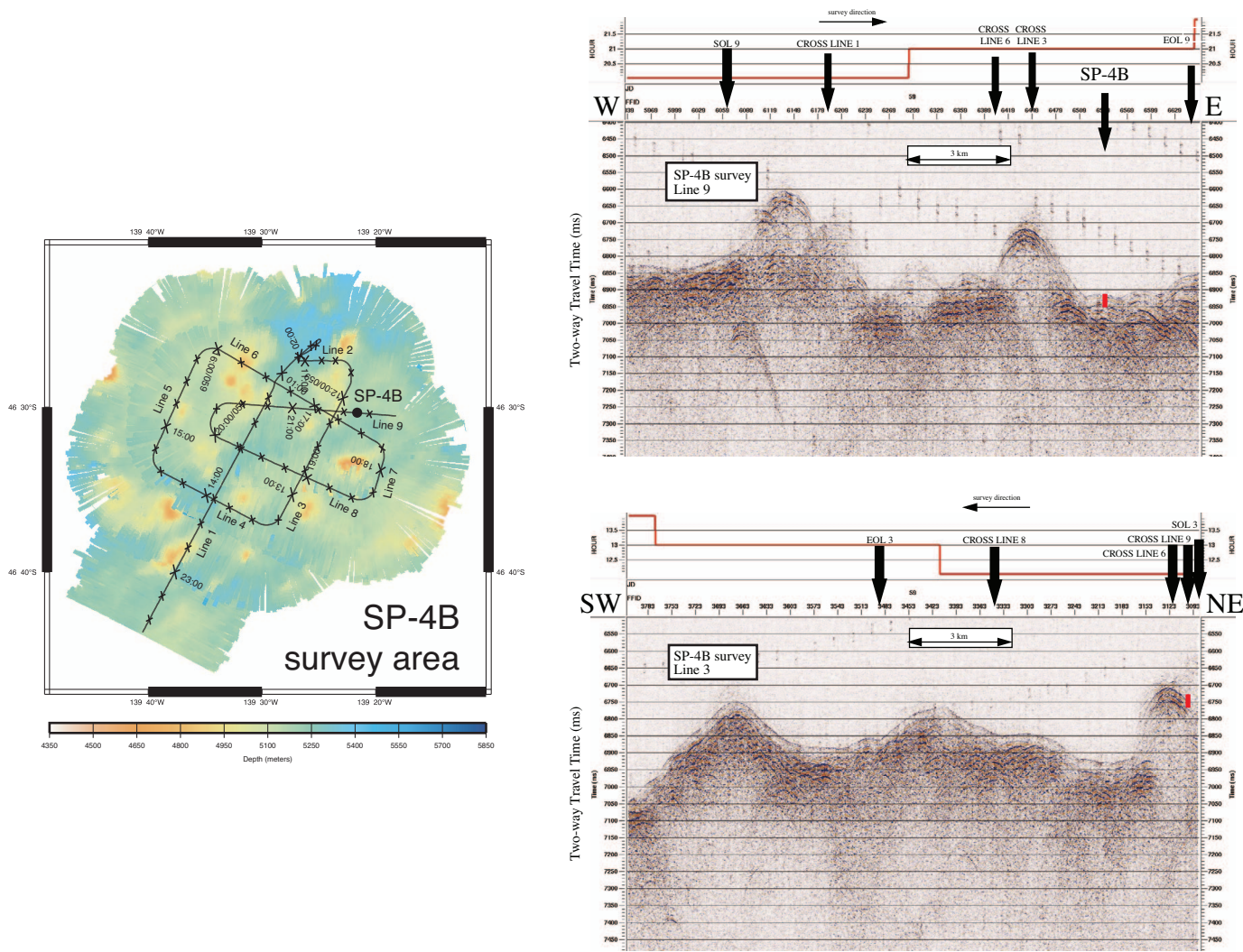
Figure AF8. Track map and seismic profiles from crossing TUIM-03 SP4B Lines 9 and 3 for proposed Site SP-4B. Red bars = proposed site location based on seismic reflectors.
