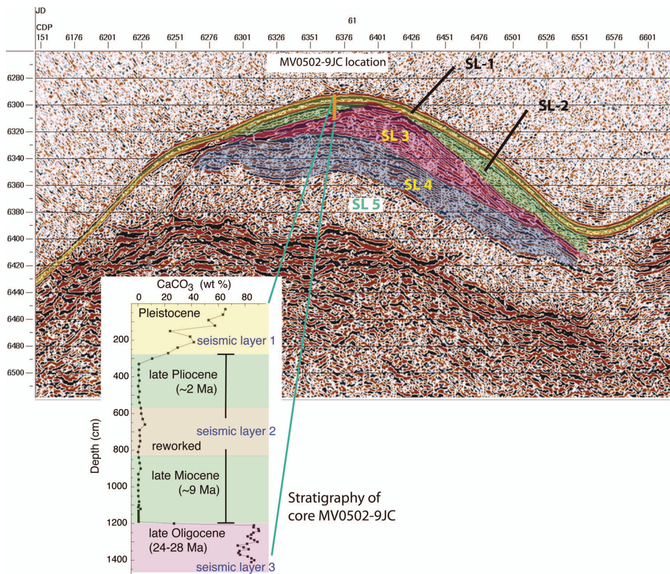
Figure F3. Seismic profile and weight percent carbonate data from piston core MV0502-9JC, 15 km northeast of proposed Site SP-14A sited along the same abyssal hill. The dramatic increase in carbonate at 12 m below seafloor is indicated by a prominent seismic reflection. CDP = common depth point. SL = seismic layer.
