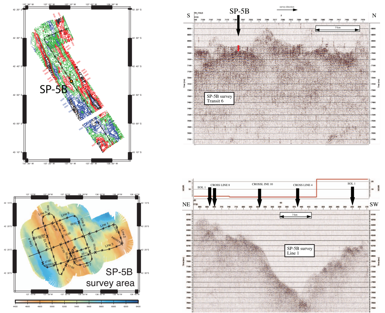
Figure AF9. Track map and seismic profiles from crossing TUIM-03 SP5B Line 1 and transit track map and transit Line 6 for proposed Site SP-5B. Red bar = proposed site location on transit line.
