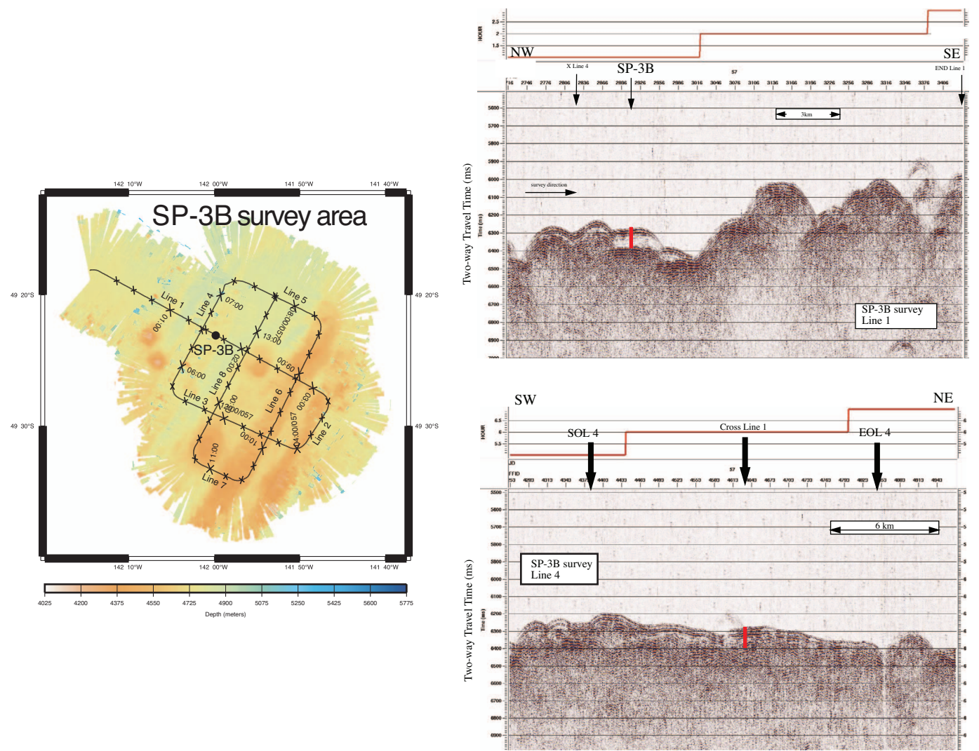
Figure AF5. Track map and seismic profiles from crossing TUIM-03 SP3B Lines 1 and 4 for proposed Site SP-3B. Red bar = proposed site location based on seismic reflectors.
