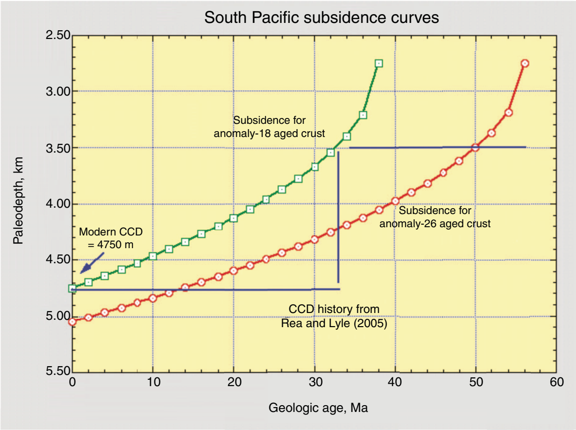
Figure F4. Crustal subsidence curves for late Eocene and late Paleocene crust shown with likely carbonate compensation depth (CCD) history. The modern CCD is from the R/V Melville site survey cruise.
