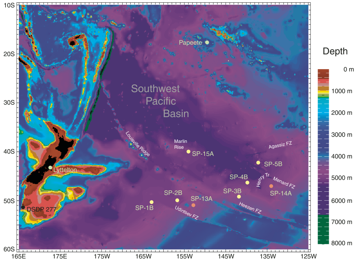
Figure F1. Map of Expedition 378 proposed drill sites. Yellow circles = sites on 56 Ma crust, orange circles = sites on 40 Ma crust, black circle = DSDP Site 277, light blue circles = ports.
