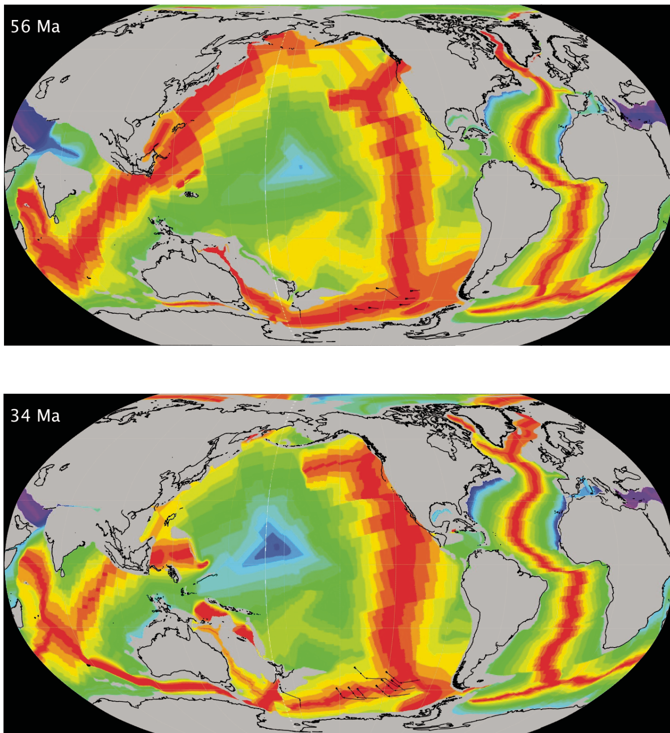
Figure F2. Paleogeographic reconstructions for 56 and 34 Ma indicating the ancient locations of Expedition 378 proposed drill sites (maps generated from GPlates).
