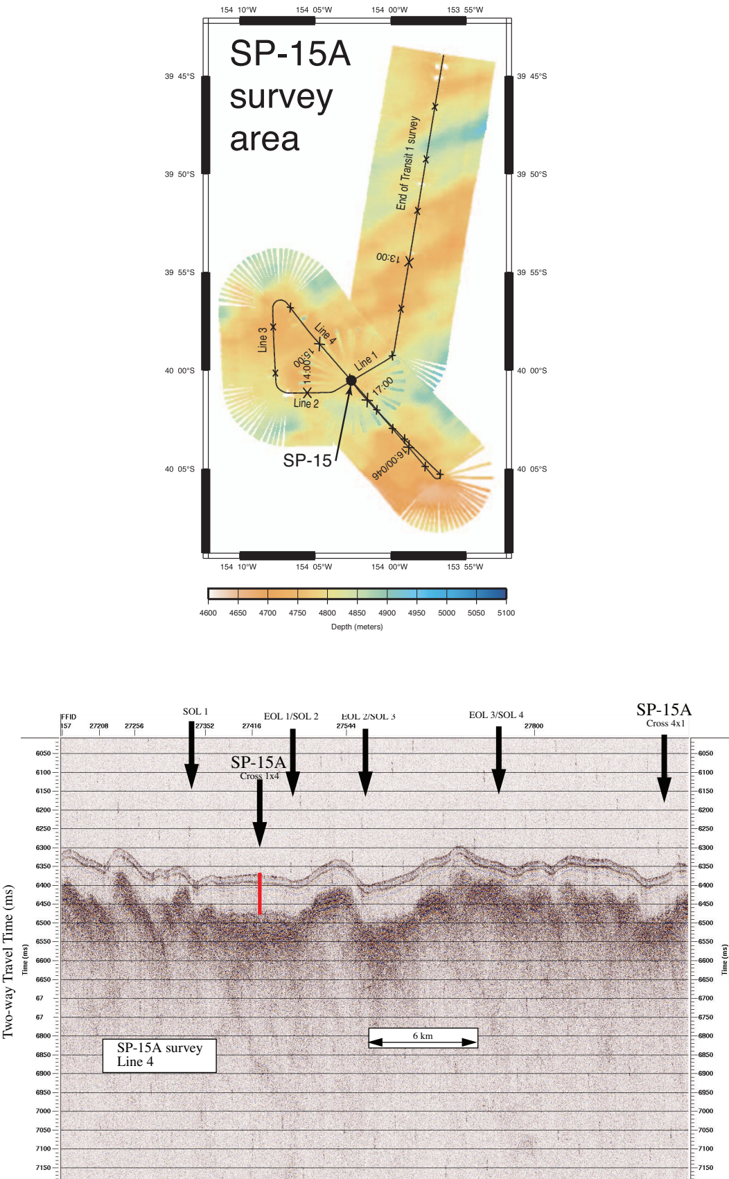
Figure AF7. Track map and seismic profile from the crossing TUIM-03 SP15A Lines 1 and 4 for proposed Site SP-15A. Red bar = proposed site location based on seismic reflectors.
