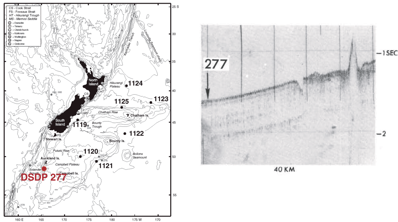
Figure AF1. Map adapted from ODP Leg 181 (Shipboard Science Party, 1999b). Shallow subbottom profiler record of proposed Site DSDP 277 from Shipboard Scientific Party (1975).
