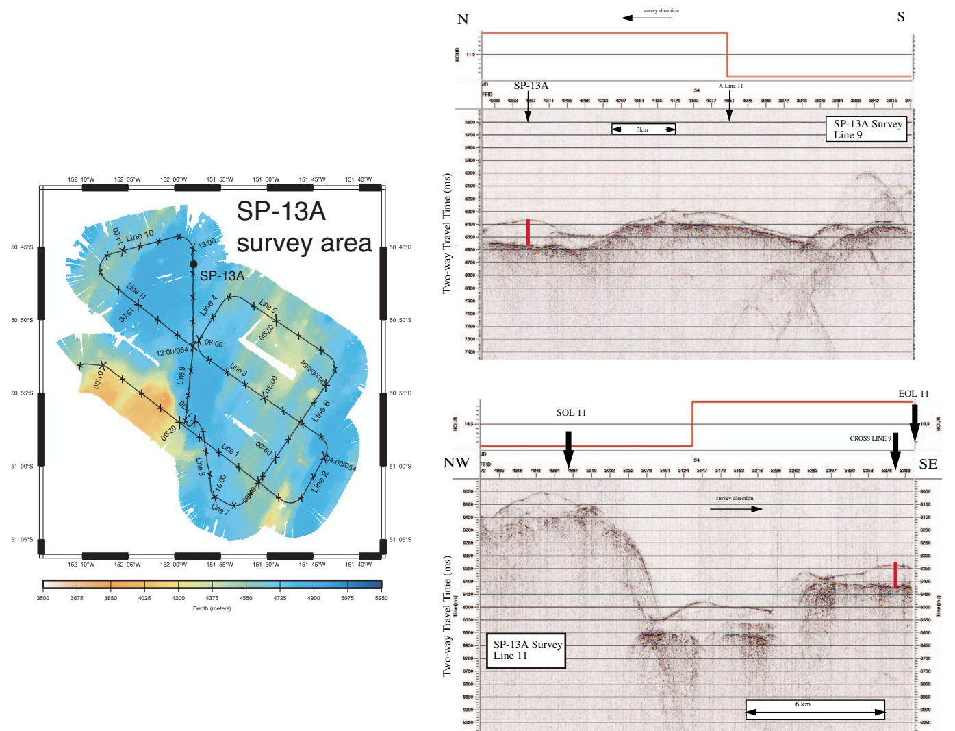
Figure AF4. Track map and seismic profiles from FFD 4340 on crossing TUIM-03 SP13A Line 9 and crossing TUIM-03 SP13A Line 11 for proposed Site SP-13A. Red bars = proposed site location based on seismic reflectors.
