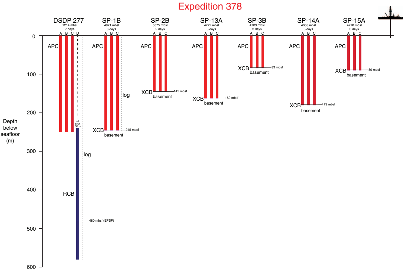
Figure F5. Planned drilling strategy for Expedition 378. APC = advanced piston coring system, RCB = rotary core barrel system, XCB = extended core barrel system. EPSP = Environmental Protection and Safety Panel.
