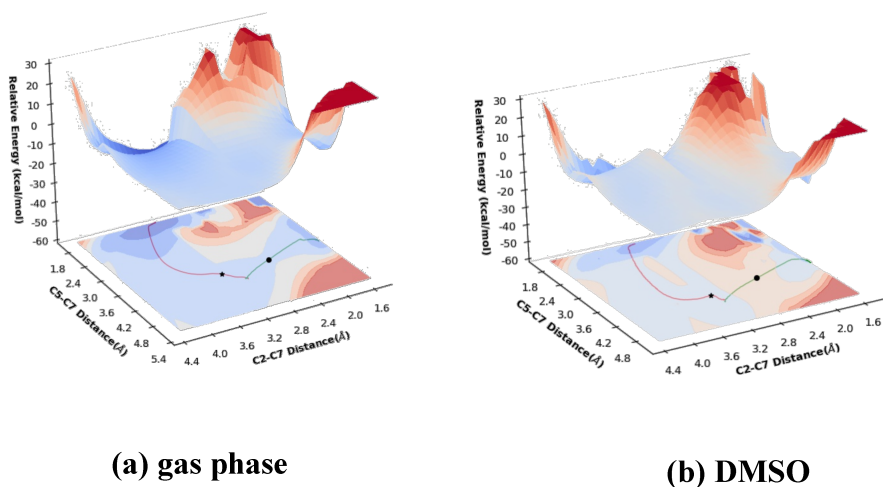
Figure 5. Potential energy surfaces: (a) M06-2X/6-311G(d), (b) PCM(DMSO)-M06-2X/6-311G(d). IRCs for TS-a are shown as red lines and IRCs for TS-b are shown as green lines. TS-a and TS-b are indicated as stars and circles, respectively.
