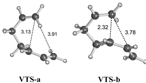
Figure 4. Geometries of variational transition states. Selected distances are shown in Å.
