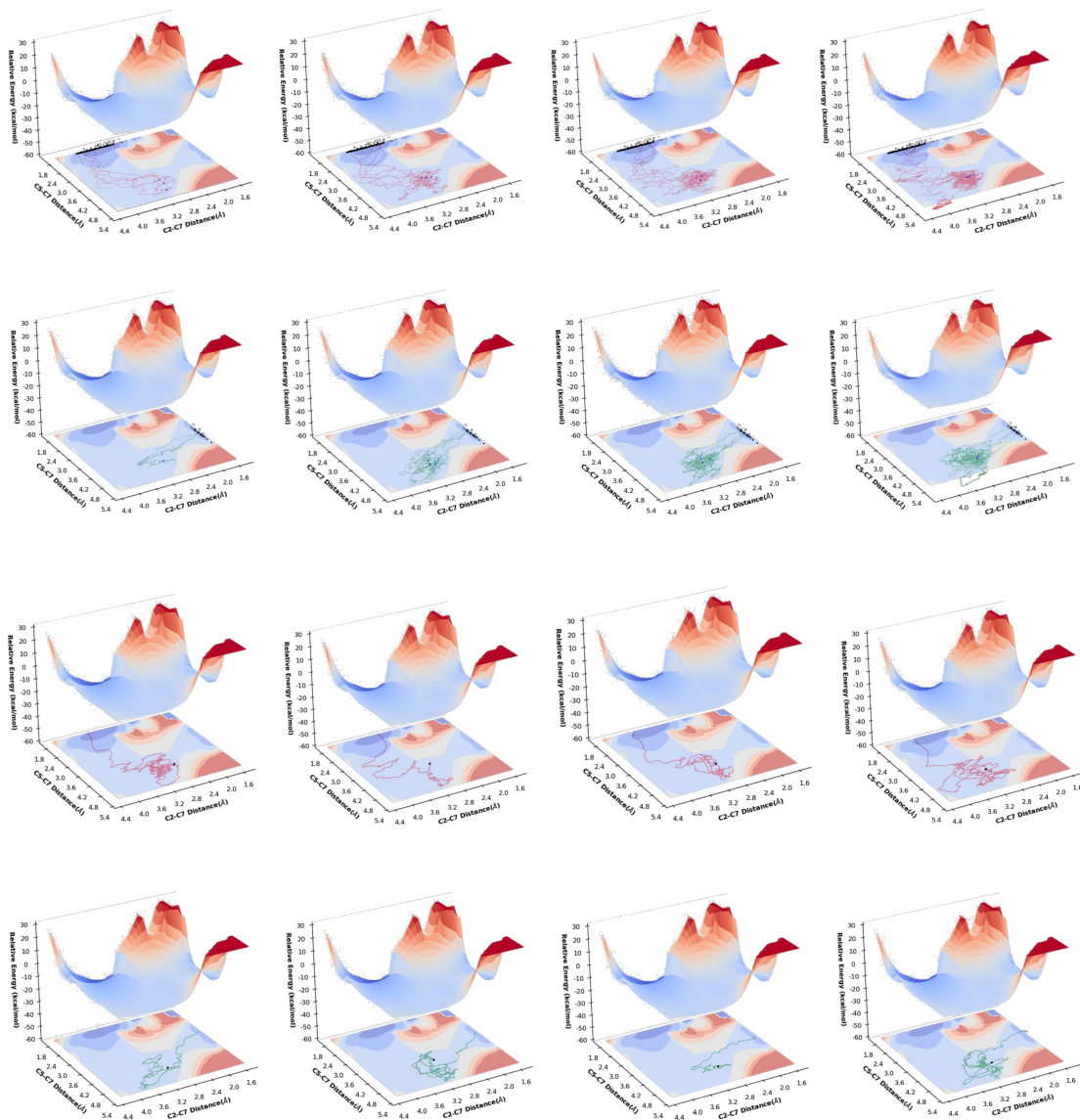
Figure 6. (1) Projections of trajectories onto the M06-2X/6-311G(d) PES, based on trajectory length (time). Left to right: 0-500 fs, 500-1000 fs, 1000-1500 fs, 1500-2000 fs. The first row corresponds to Prod-1 -forming trajectories. The second row corresponds to Prod-2 -forming trajectories. (2) Projections of representative “turn back” trajectories onto the M06-2X/6-311G(d) PES. The third row shows representative Prod-1 -forming “turn back” trajectories. The bottom row shows representative Prod-2 -forming “turn back” trajectories.
