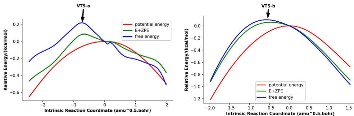
Figure 3. Reaction coordinate plots for pathways a (left) and b (right). The locations of VTS-a and VTS-b are highlighted.
