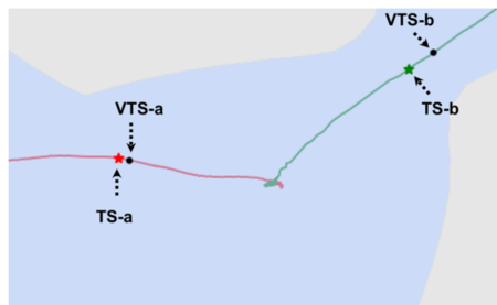
Figure 7. Close-up view of the reactant region of the surface from Figure 5a.
