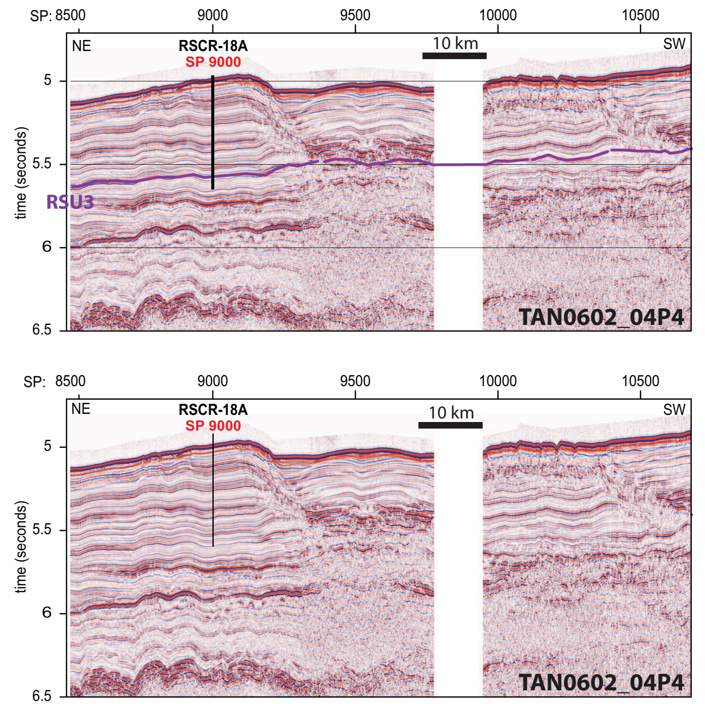
Figure AF24. Seismic reflection profile Line TAN0602-04P4 with location of proposed alternate Site RSCR-18A (73.910571°S, 162.456325°W; SP9000; water depth = 3650 m; target depth = 650 mbsf; approved maximum penetration = 650 mbsf).
