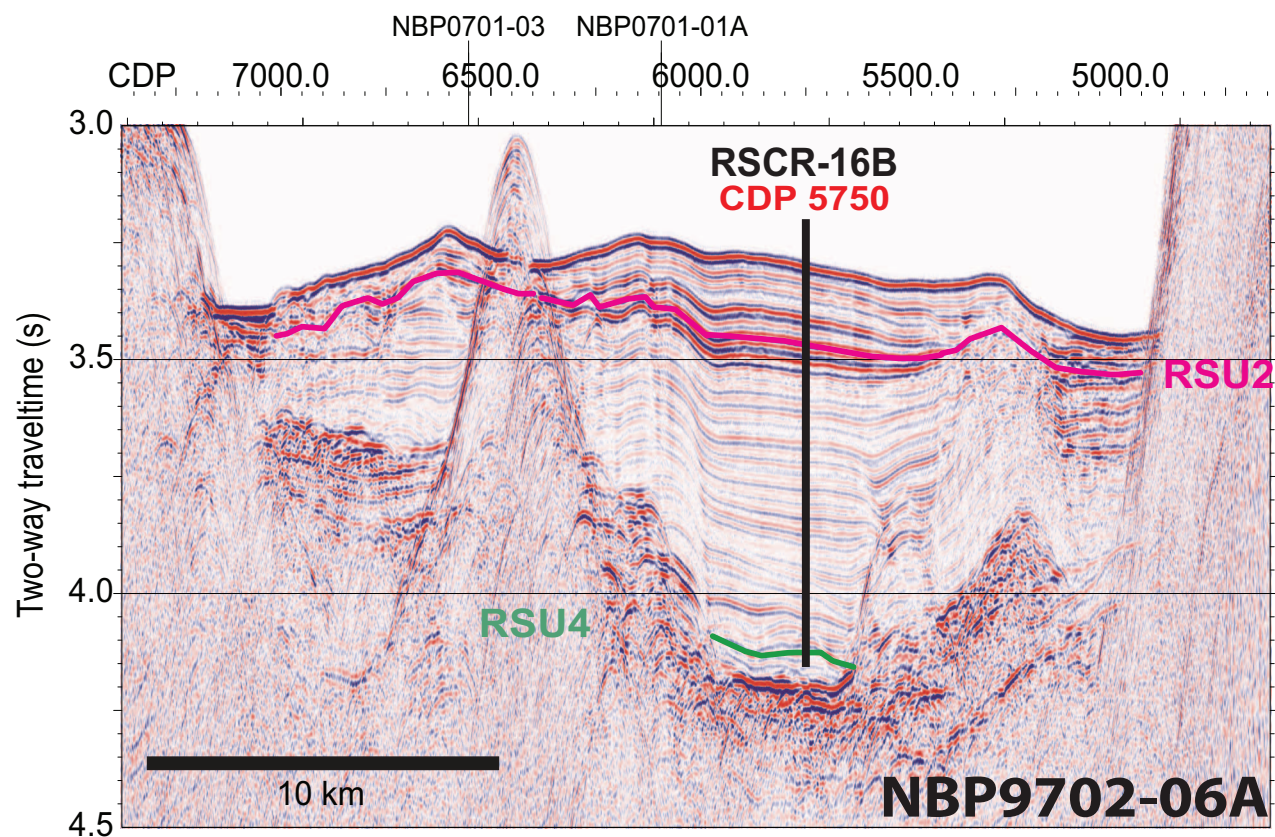
Figure AF21. Seismic reflection profile Line NBP9702-06A with location of proposed alternate Site RSCR-16B (70.59171889°S, 172.91573501°E; CDP5750; water depth = 2340 m; target depth = 950 mbsf; approved maximum penetration = 950 mbsf). CDP = common depth point.
