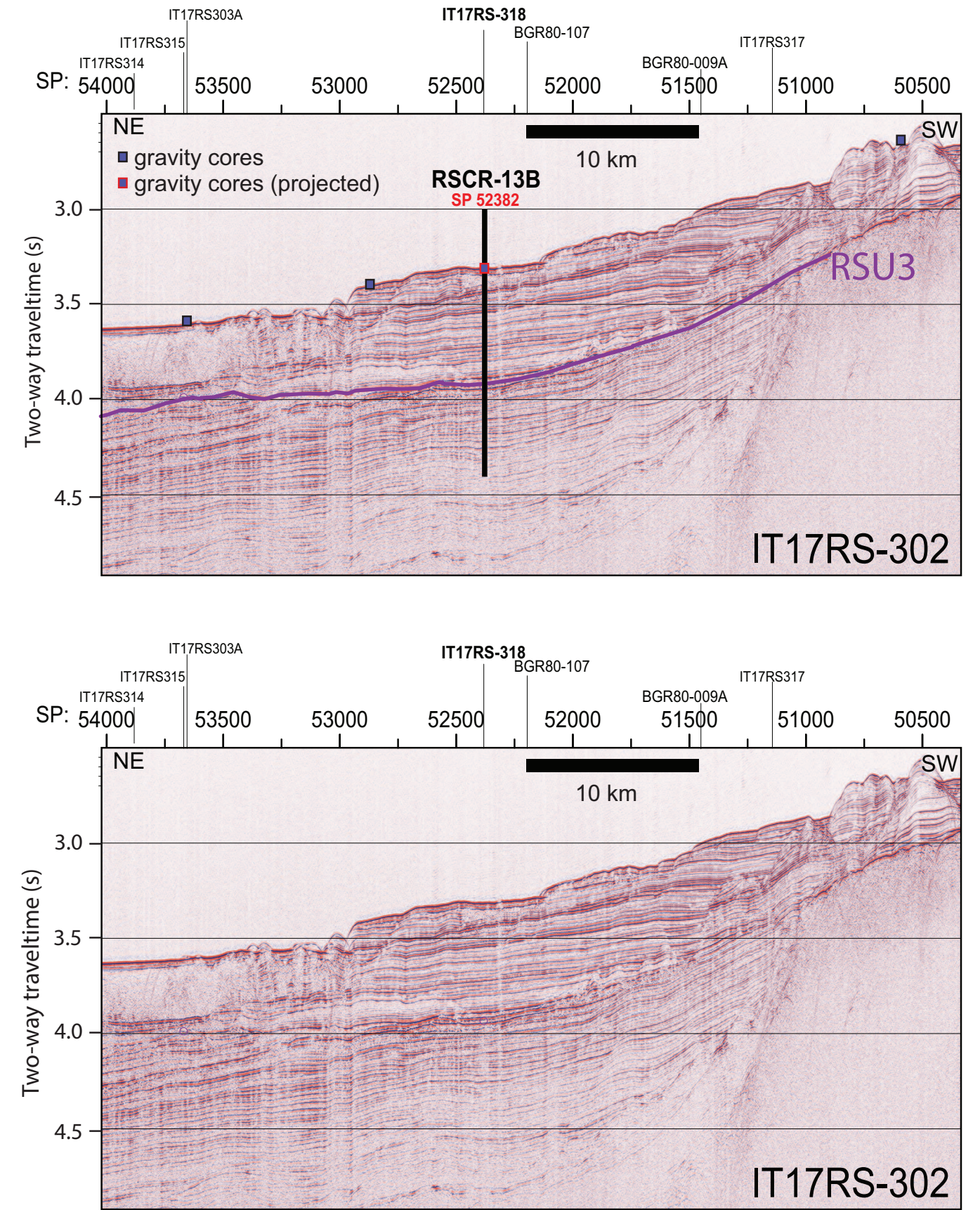
Figure AF15. Seismic reflection profile Line IT17RS-302 with location of proposed alternate Site RSCR-13B (73.9175423°S, 175.349974°W; SP52382; water depth = 2390 m; target depth = 1000 mbsf; approved maximum penetration = 1000 mbsf).
