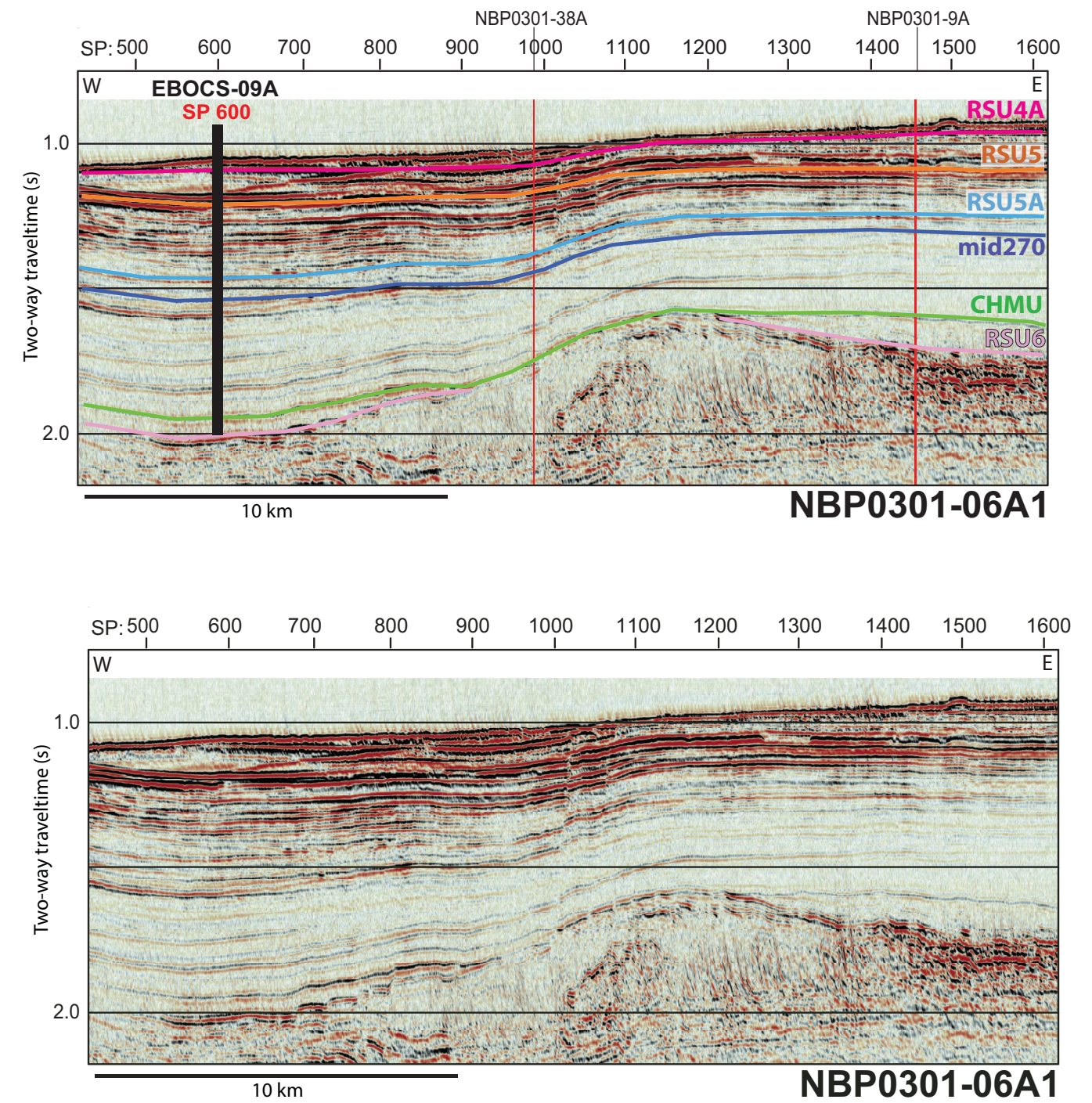
Figure AF4. Seismic reflection profile Line NBP0301-06A with location of proposed alternate Site EBOCS-09A (77.247108°S, 171.622215°; SP600; water depth = 764 m; target depth = 1300 mbsf; approved maximum penetration = 1300 mbsf).
