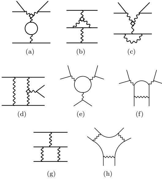
FIG. 5. Feynman diagrams contribute to the beta equation of the six-point vertex.
