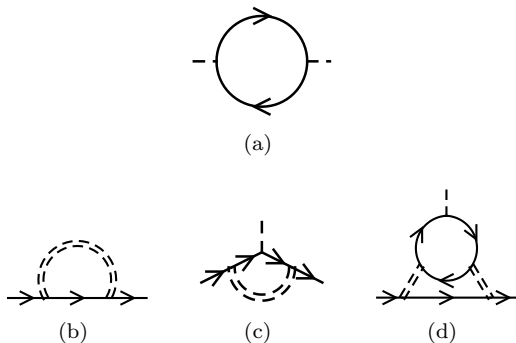
FIG. 2. (a) The polarization of the scalar field. The solid line (single-dashed) represents the Dirac fermion propagator (the bare scalar propagator). (b-d) The 1/N order Feynman diagrams. The double-dashed line represents the screened scalar propagator.
