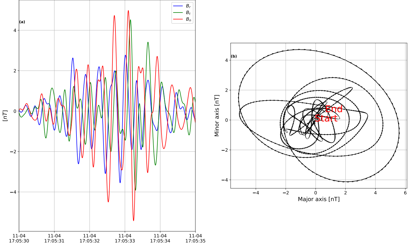
Figure 11. a) Waveforms of magnetic field components in the RTN frame recorded in a close vicinity of the leading edge of the structure shown in Figure 9. b) Hodograph of the magnetic field in the plane transverse to the wave normal vector.
