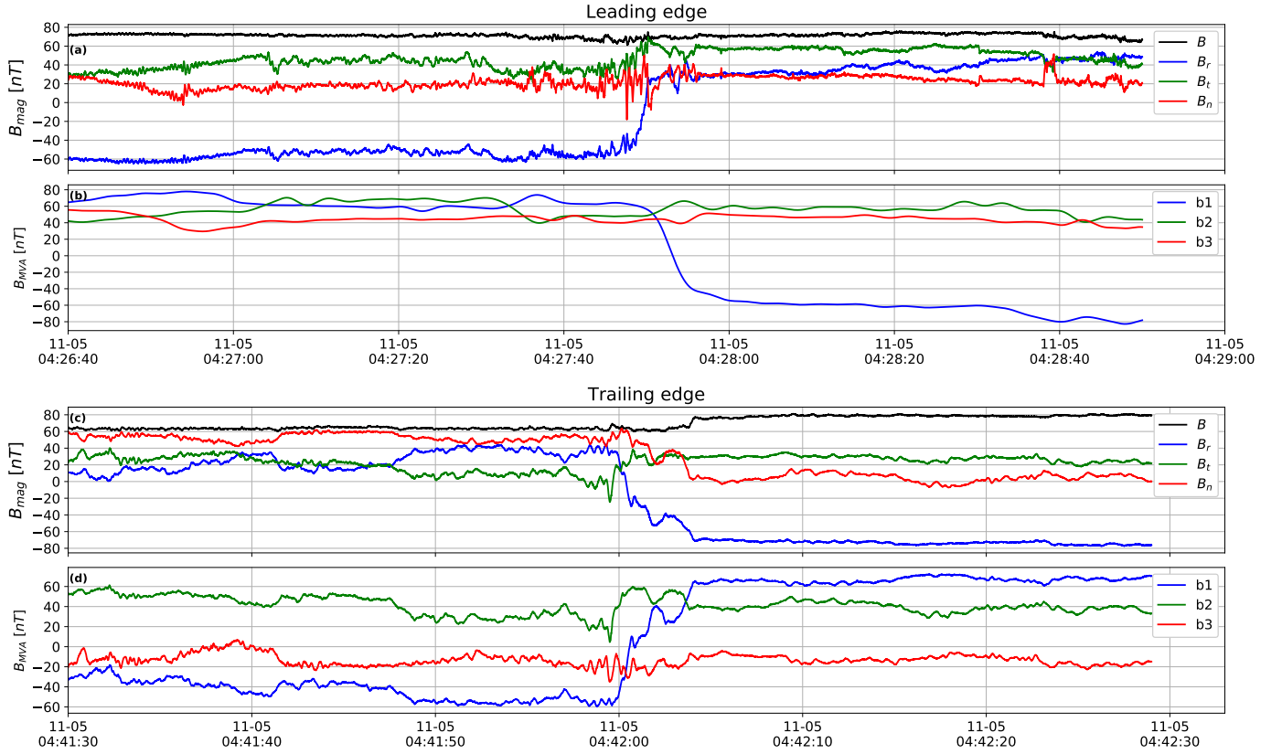
Figure 17. The magnetic field on the structure boundaries: the magnetic field components on the leading edge in the RTN frame (a) and in the MVA frame (b); the magnetic field components on the trailing edge in the RTN frame (c) and in the MVA frame (d).
