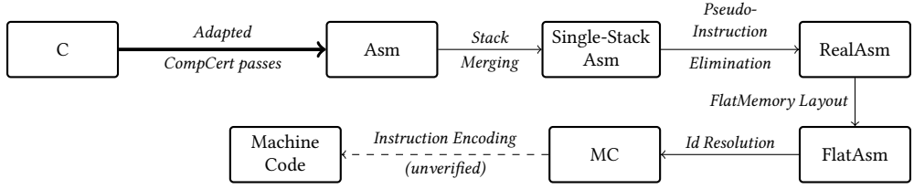
Fig. 4. Stack-Aware CompCert
