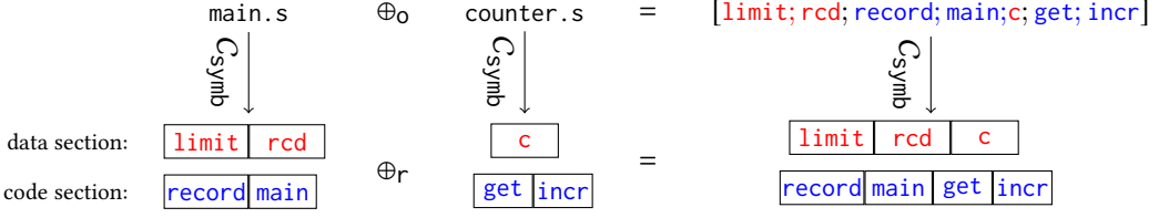
Fig. 13. An Example of Commutativity for Symbol Table Generation using \oplus_0
