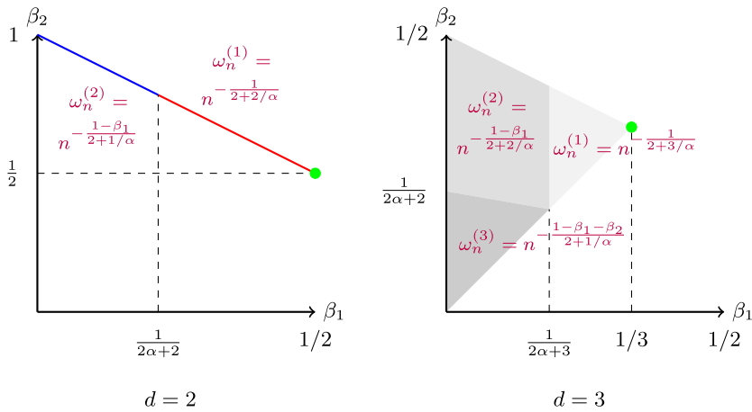
FIG. 2. Phase transitions of the local rate of convergence for the \beta -fixed lattice design in d = 2 (left panel, in the line segment \{\beta_1 \leq 1/2, \beta_2 = 1 - \beta_1\} ) and d = 3 (right panel, in the triangle \{\beta_1 \leq 1/3, \beta_1 \leq \beta_2 \leq (1 - \beta_1)/2\} ). \omega_n^{(\ell)} = local rate with \kappa_* = \ell . Local rates in fixed lattice and random design cases match for \kappa_* = 1 . Green points = values of (\beta_1, \beta_2) for the balanced fixed lattice design.
