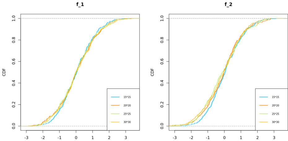
FIG. 3. Empirical cumulative distribution functions for n^{1/4}(\hat{f}_n(x_0) - f_i(x_0)) ( i = 1, 2 ) based on B = 300 repetitions. Here, d = 2 , f_1(x_1, x_2) = e^{x_1+x_2} in the left panel and f_2(x_1, x_2) = e(x_1 + x_2) in the right panel, and x_0 = (1/2, 1/2) . Lattice sizes: 15 \times 15 , 20 \times 20 , 25 \times 25 , 30 \times 30 .
