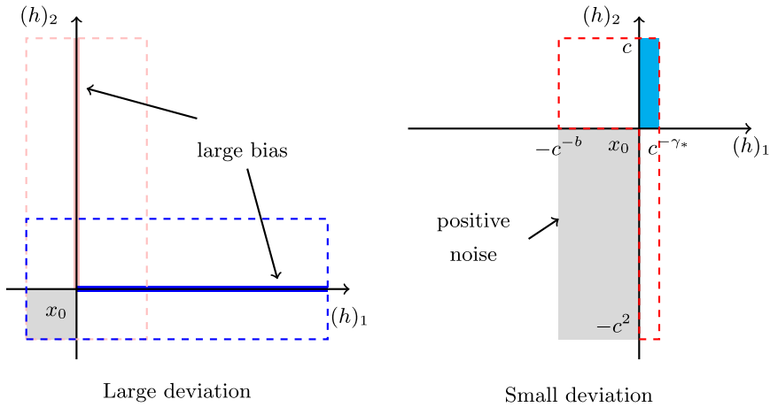
FIG. 5. Proof outlines: Large and small deviation problems.
