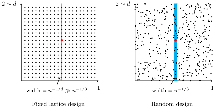
FIG. 1. Illustration of the oracle estimator in the balanced fixed lattice and random design cases. Horizontal direction = dimension 1. Vertical direction = dimensions 2 to d . Red point = x_0 . Blue strip = samples over which the oracle estimator takes the average.
