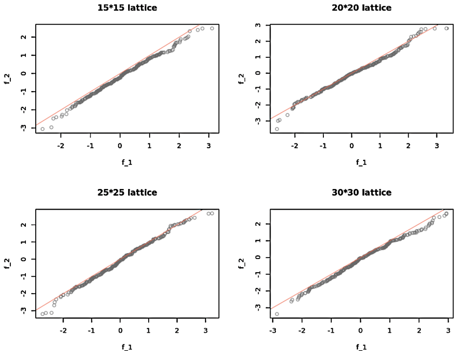
FIG. 4. QQ-plots for the distributions of n^{1/4}(\hat{f}_n(x_0) - f_1(x_0)) (horizontal) versus n^{1/4}(\hat{f}_n(x_0) - f_2(x_0)) (vertical) based on the same simulation as in Figure 3. Lattice sizes: 15 \times 15 , 20 \times 20 , 25 \times 25 , 30 \times 30 .
