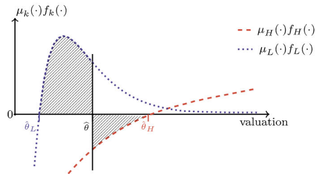
Fig. 1. Weighted virtual valuations for low-type (dotted line) and high type (dashed line) buyer around \hat{\theta} . The shaded areas correspond to the virtual revenue that the seller misses when using a static contract with respect to the case in which the interim types are public information.
