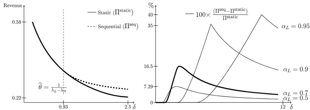
Fig. 5. Left : Optimal expected revenue for static and sequential. Right : Percentage improvement of the sequential over the static contract. In both figures we set \lambda_L = \lambda_H + \delta with \lambda_H = 0.5 . In the left figure, we set \alpha_L = 0.7 , while in the right figure, \alpha_L takes values in \{0.5, 0.7, 0.9, 0.95\} .
