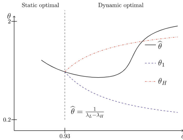
Fig. 4. Optimal thresholds for static and sequential contracts when setting \lambda_L = \lambda_H + \delta , with \alpha_L = 0.7 and \lambda_H = 0.5 .
