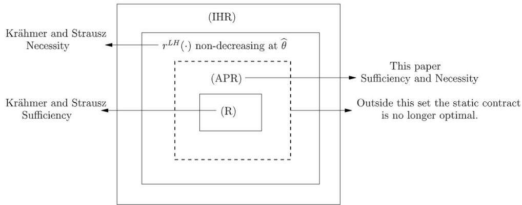
Fig. 3. Optimality of the static contract for (IHR) distributions, with K = 2 and a single buyer.
