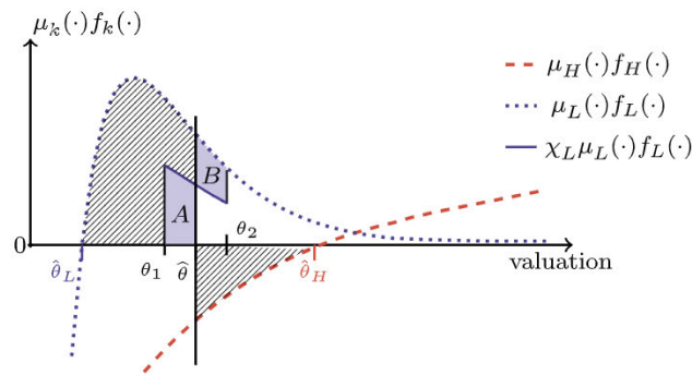
Fig. 2. Weighted virtual valuations for low-type (dotted line) and high-type (dashed line) buyers around \hat{\theta} . The shaded areas correspond to the virtual revenue that the seller leaves on the table when using a static contract with respect to the case in which the interim types are public information. We display the deviation from the static contract for the low-type (solid line). If the solid areas A and B are such that A - B \geq 0 , the deviation is profitable.
