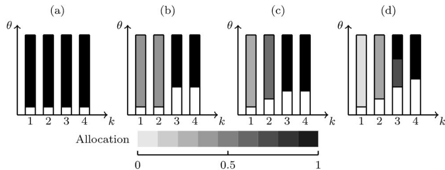
Fig. 6. Optimal allocations for K = 4 ; types have exponential distributions with means (2.2, 5.0, 12, 50) (for numerical simplicity, we use truncated versions of these distributions in the interval [0, 60] ). In each panel the vertical axis corresponds to buyers' valuations, and the horizontal axis corresponds to the interim type. Each bar represents the allocation for each type; lighter gray indicates lower probability of allocation, while darker gray indicates a higher probability of allocation. White represents no allocation and black full allocation. From panels (a) to (d), the fractions, \alpha_k , for each type are (0.7, 0.2, 0.05, 0.05), (0.4, 0.1, 0.4, 0.1), (0.3, 0.2, 0.4, 0.1) and (0.25, 0.25, 0.1, 0.4), respectively.
