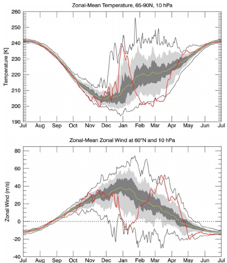
Figure 1. 10-hPa 65–90° N ERA-Interim reanalysis (Dee et al., 2011) zonal-mean temperatures (top) and zonal-mean zonal wind at 60°N (bottom) for July 2018 to June 2019 (red lines). An SSW event is seen as the upward spike in temperature and the reduction to less than 0 m/s in zonal wind (easterlies). The yellow lines signify the daily average conditions in the stratosphere for that time of year, while the gray shading shows 30th/70th (dark) and 10th/90th (light) percentiles. Solid black lines show the daily max/min for prior winters 1979–2018. The month ticks indicate the first day of the month.
