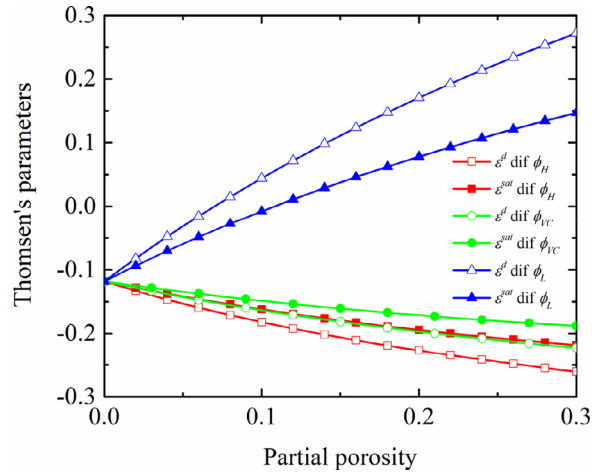
Fig. 5. The effect of the variation of the partial porosities on mesoscopic anisotropic Thomsen's parameters of dry bone ( \epsilon^d ) and that of saturated bone ( \epsilon^{sat} ).
