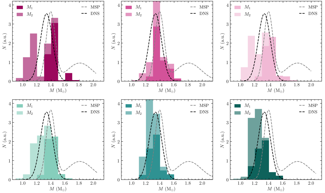
Figure 9. Scaled mass distributions for each EOS choice, weighted by the [\text{Eu}/\text{Fe}] distributions of RPA measurements. Each panel indicates separate EOSs, using the same order and colors as in Figure 8. The contribution to the total mass distribution by the primary ( M_1 ) and secondary ( M_2 ) NSs are indicated by color shading. The gray and black dashed curves show the fitted mass distributions for NSs in DNS and MSP systems (see text for details).
