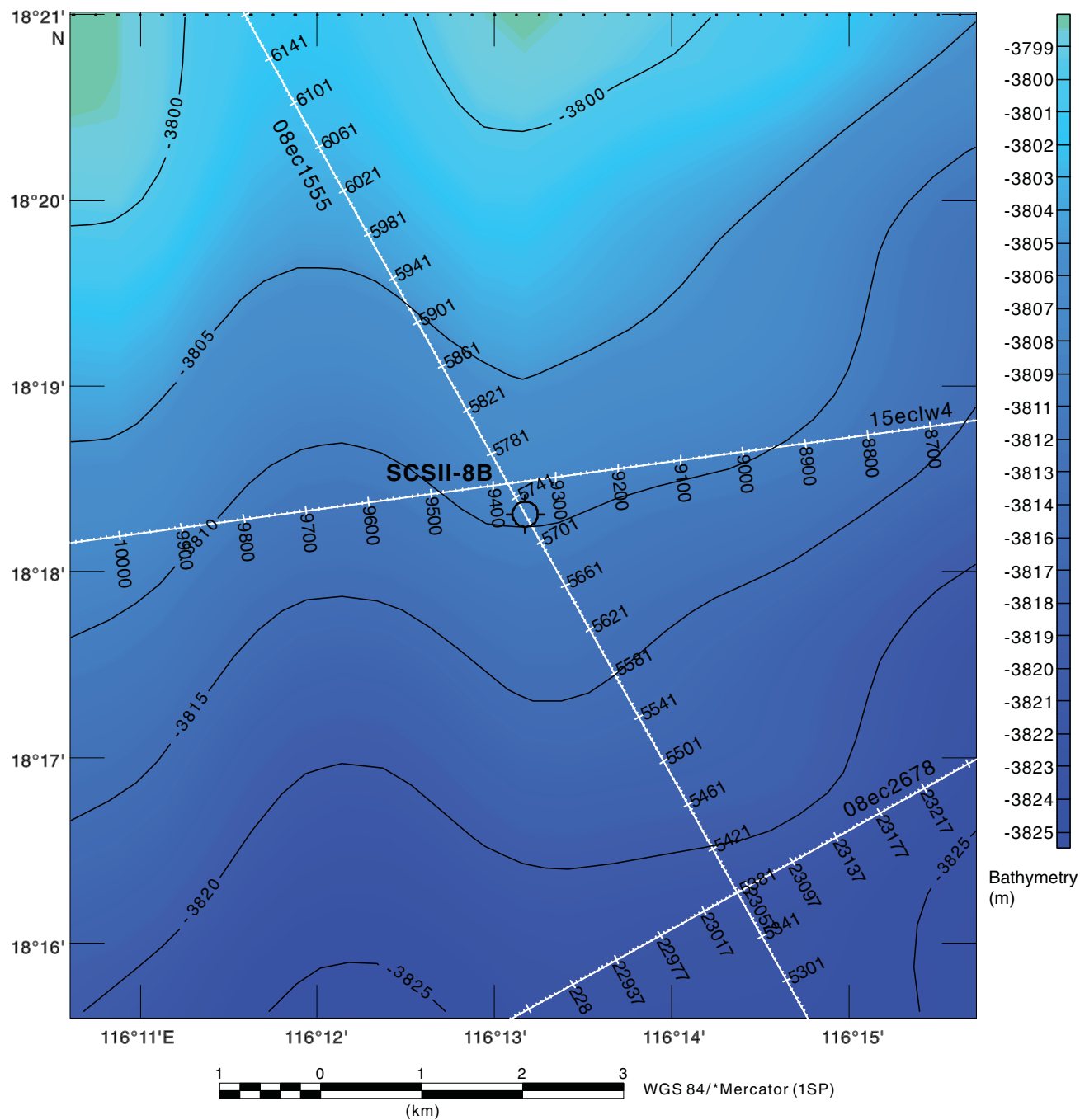
Figure AF21. Bathymetry, proposed Site SCSII-8B.
