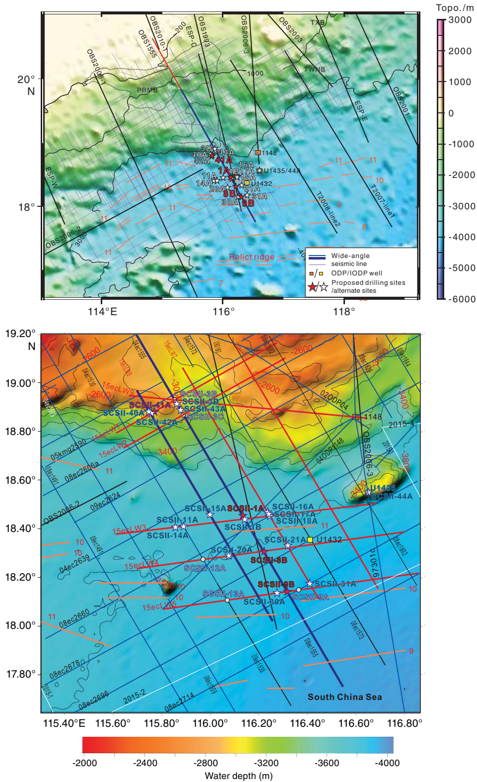
Figure F2. Northern South China Sea rifted margin with seismic coverage of 2-D, time-migrated multichannel seismic reflection seismic data and ocean-bottom seismometer data (3-D data not shown). Key seismic lines used for planning of the drilling transect are marked in thick blue and shown in Figures F3 and F4. Proposed Expedition 367/368 drill sites are shown (red solid stars = primary proposed sites, white stars = alternate proposed sites). Previous ODP Leg 184 and IODP Expedition 349 sites are shown as orange or yellow squares. Magnetic lineations within the ocean crust are shown in red with interpreted chrons after Briais et al. (1993).
