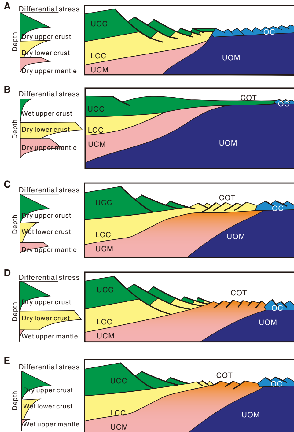
Figure F8. A–E. Composite figures redrawn from models in Huismans et al. (2011), Sibuet and Tucholke (2012), Makris et al. (2012), and Sun et al. (2016) showing the spectrum of possible magma-poor rifted margin models that can be tested with the proposed drilling transect. The variations in the models are due to different initial rheologies in the upper and lower crust and in the upper mantle; these rheologic differences cause variations in stretching of the various lithospheric layers. Model in D features a strong lower crust overlying a weak, wet upper mantle, resulting in upper subcontinental (serpentinized) mantle dominating the continent–ocean transition (COT). A particularly interesting alternative is shown in C, in which moderately weaker lower crust leads to its exhumation in the COT. UCC = upper continental crust, LCC = lower continental crust, UCM = upper continental mantle, UOM = upper oceanic mantle, OC = oceanic crust.
