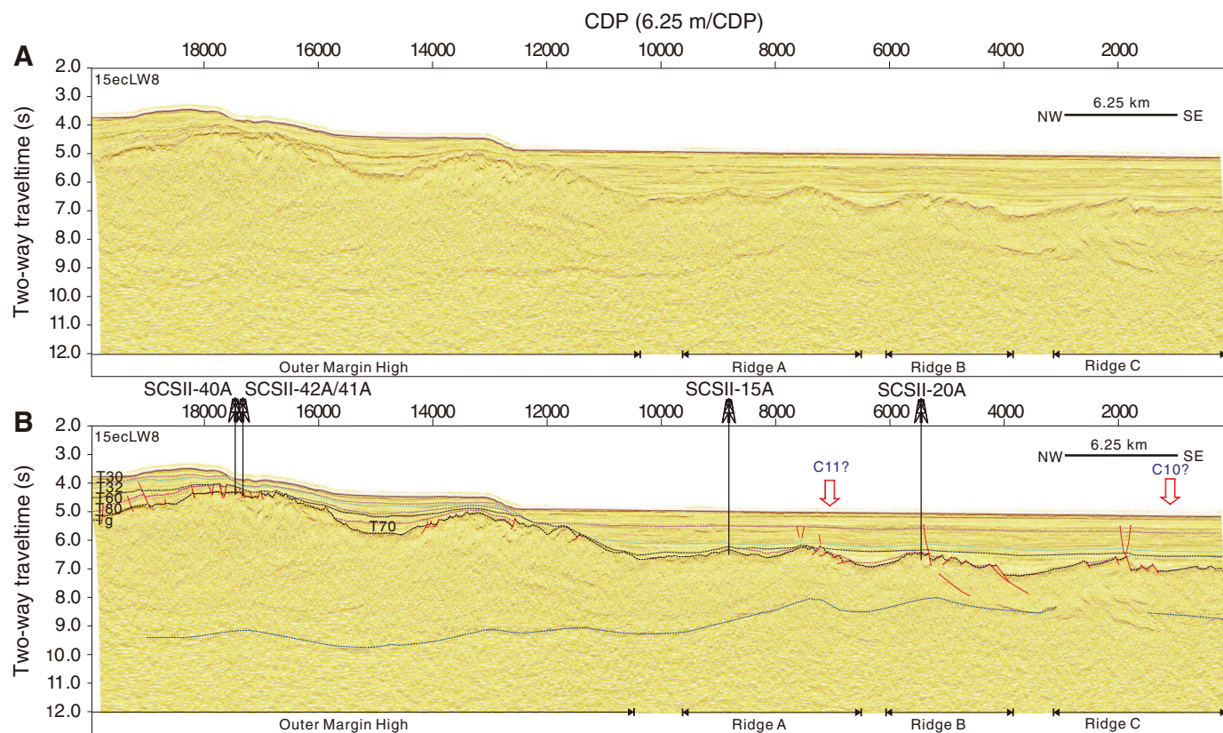
Figure F5. New (2015) deep crustal time-migrated seismic reflection Profile 15ecLW8 (A) without interpretation and (B) with interpretation. The line is located parallel to and ~12.5 km southwest of Line 1555 shown in Figures F2 and F3. The crustal structure shown by the two lines is quite similar. However, the Mohorovicic seismic discontinuity is better imaged from below the outer margin high and across the continent–ocean transition on this profile. Key seismic unconformities are shown in purple (T70; ~32 Ma) and black (T60; ~23 Ma). See also Figure F4. Tg unconformity (black) is basement. Alternate proposed drill sites are shown on this profile, but primary proposed Site SCSII-41A is located ~2 km northeast from alternate proposed Site SCSII-42A, along Line 15ecLW1 (Figures F2, F3). Data courtesy of the Chinese National Offshore Oil Corporation.
