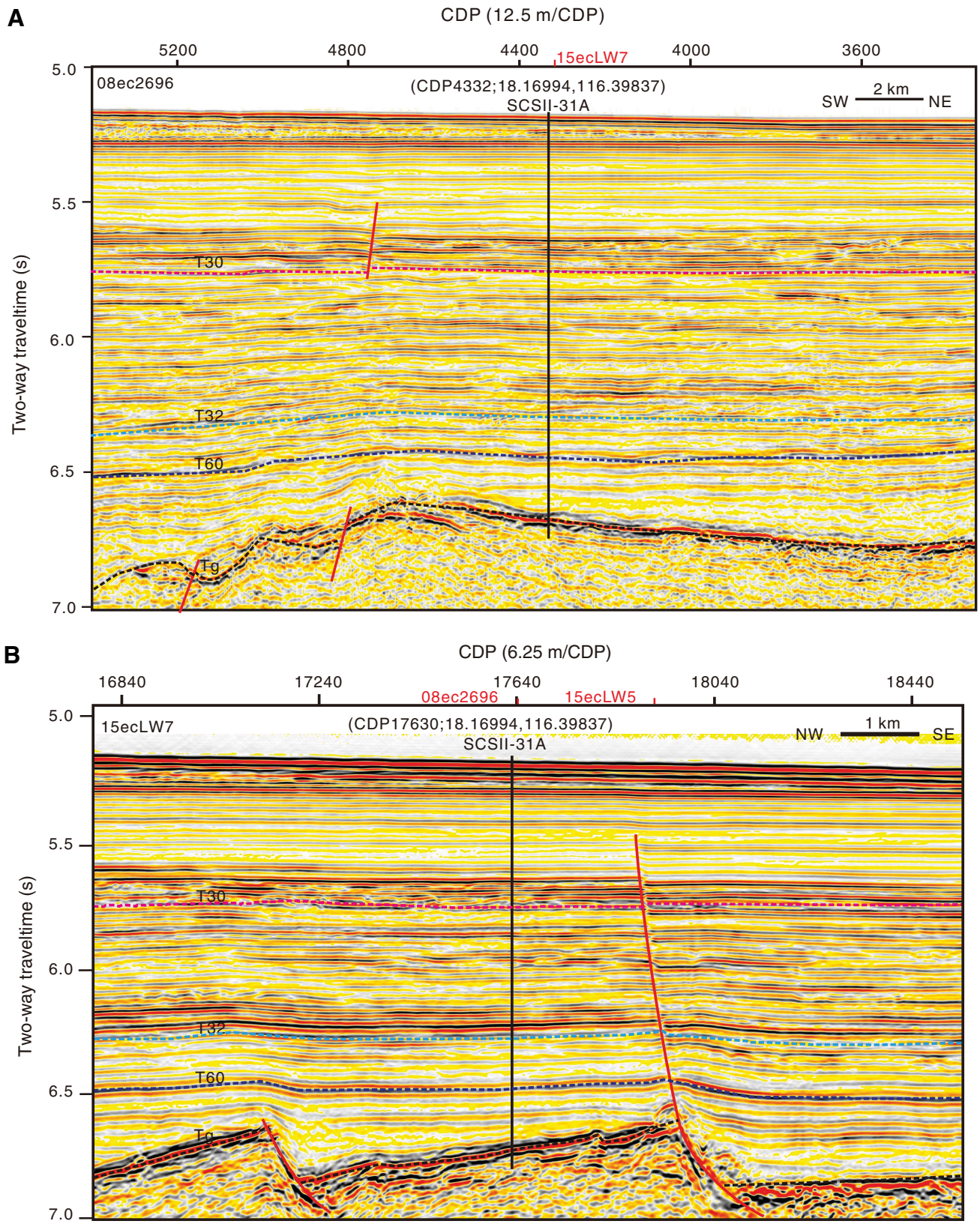
Figure AF31. (A) Primary seismic Line 08ec2696 and (B) crossing Line 15ecLW7, proposed Site SCSII-31A. CDP = common depth point. Dashed lines = unconformities, solid red lines = faults.
