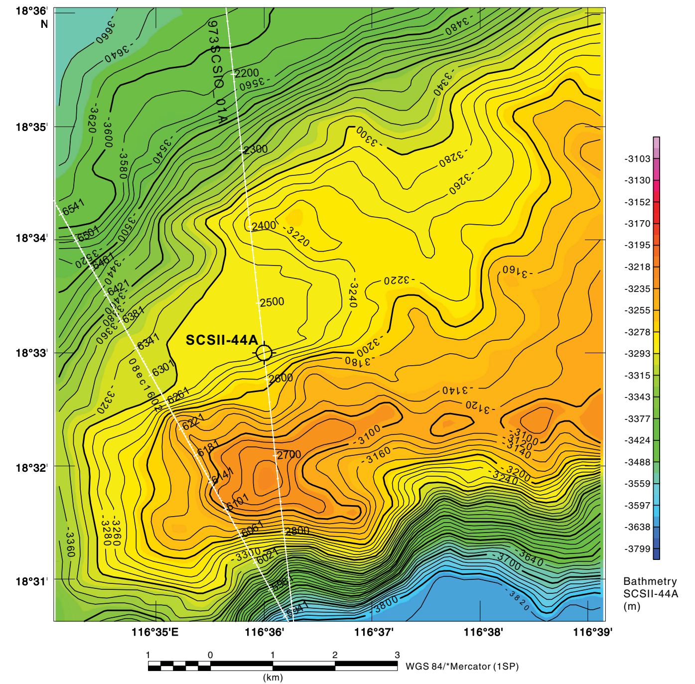
Figure AF8. Bathymetry, proposed Site SCSII-44A.
