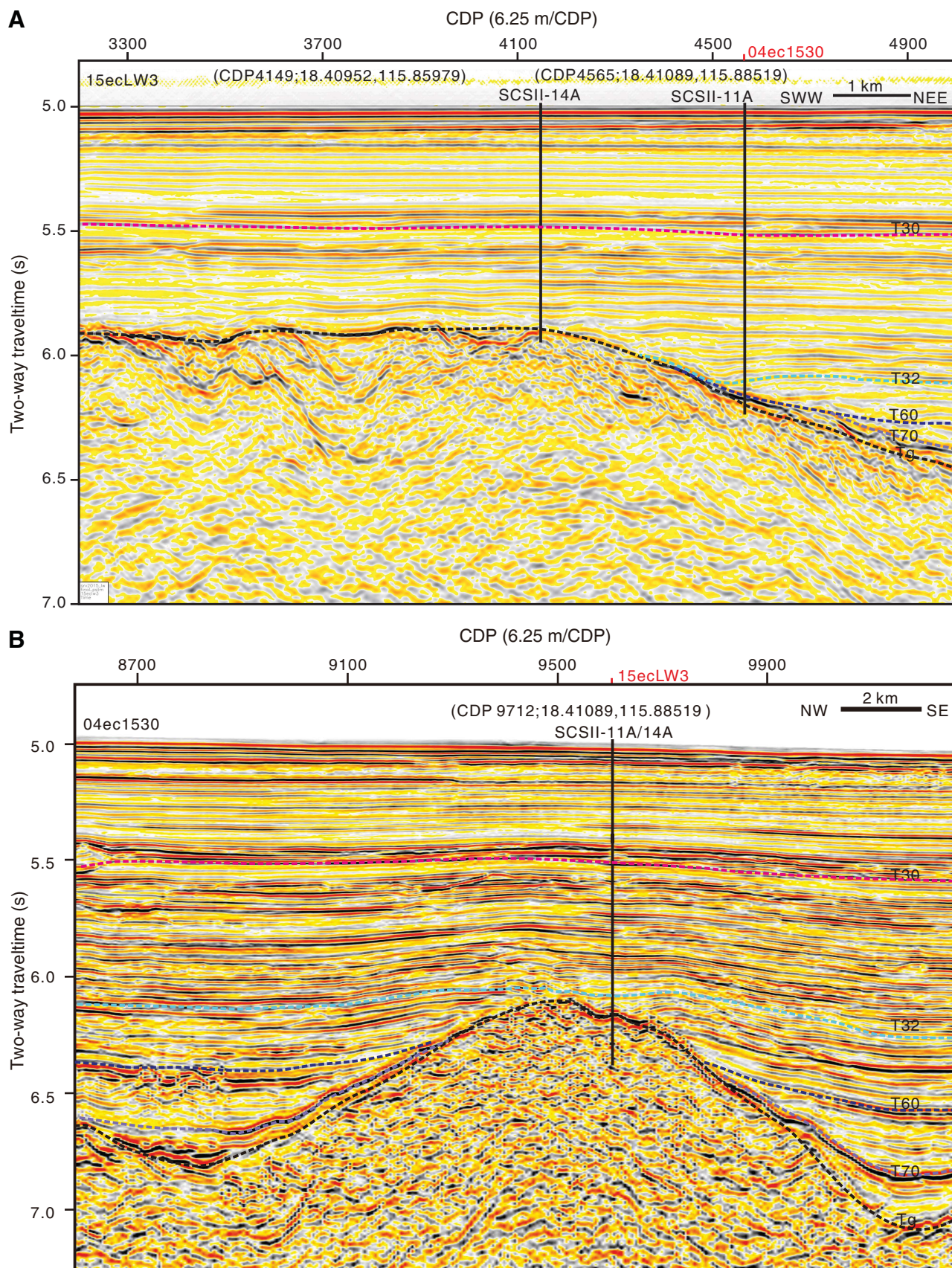
Figure AF13. (A) Primary seismic Line 15ecLW3 and (B) crossing Line 04ec1530, proposed Sites SCSII-11A and SCSII-14A. CDP = common depth point. Dashed lines = unconformities.
