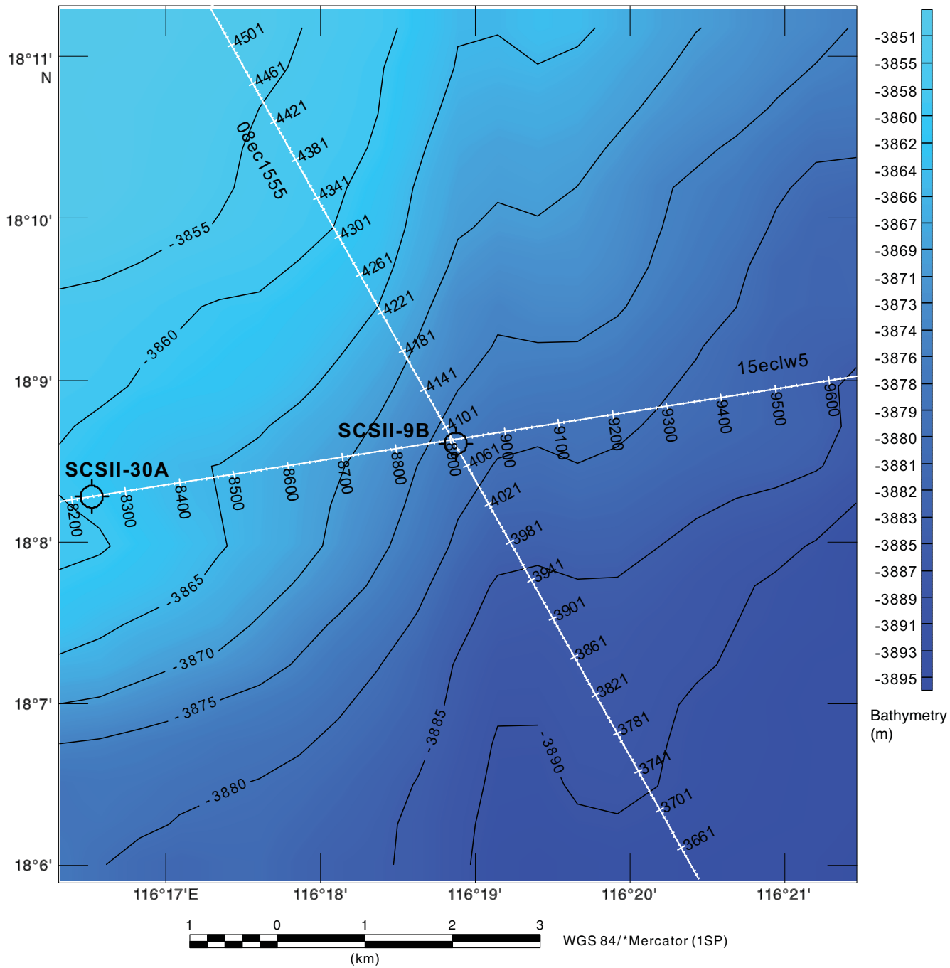
Figure AF27. Bathymetry, proposed Sites SCSII-9B and SCSII-30A.
