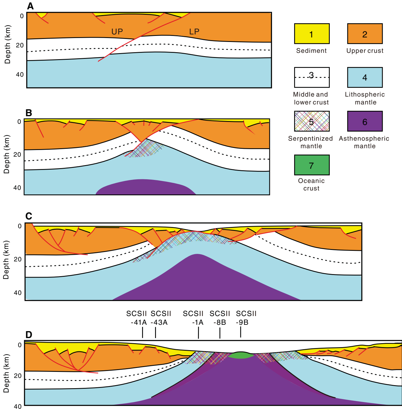
Figure F7. A–D. Schematic development of continental breakup initiated by a simple shear along a deep, low-angle fault with generalized locations of proposed drill sites (bottom). B–D are slightly modified from Huisman and Beaumont (2011) and illustrate modeling based stages of extension at magma-poor rifted margins of the Iberia-Newfoundland type. Key features of the final margin structure are thinning of the lower crust, juxtaposition of upper crustal structural units to lower crust or serpentinized mantle (proposed Site SCSII-1A), and a fairly wide zone of serpentinite crust (proposed Sites SCSII-8B and SCSII-9B?) between the outer margin and igneous oceanic crust. The northern South China Sea margin shows a striking general similarity to the left side of the upper plate margin in D. However, only sampling by drilling of the key structural units can discriminate between this and other possible models. UP = upper plate, LP = lower plate.
