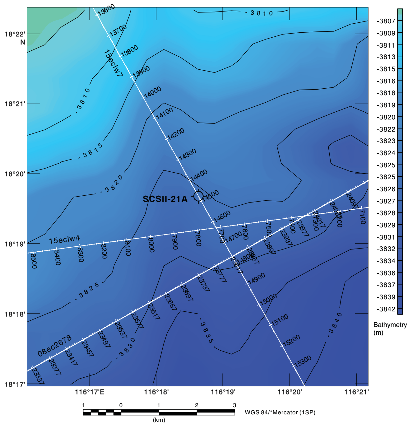
Figure AF25. Bathymetry, proposed Site SCSII-21A.
