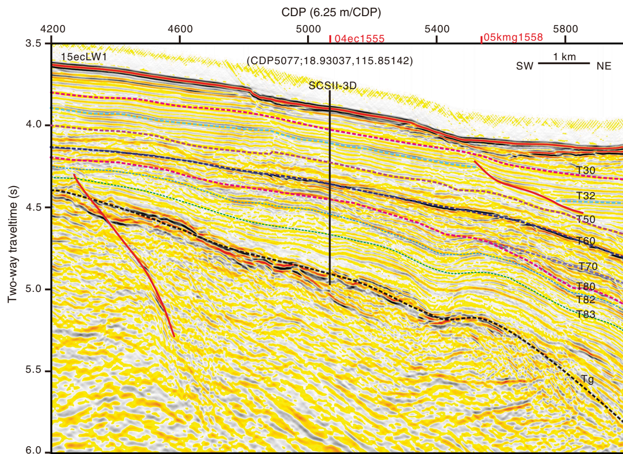
Figure AF6. Crossing seismic Line 15ecLW1, proposed Site SCSII-3D. CDP = common depth point. Dashed lines = unconformities, solid red lines = faults.
