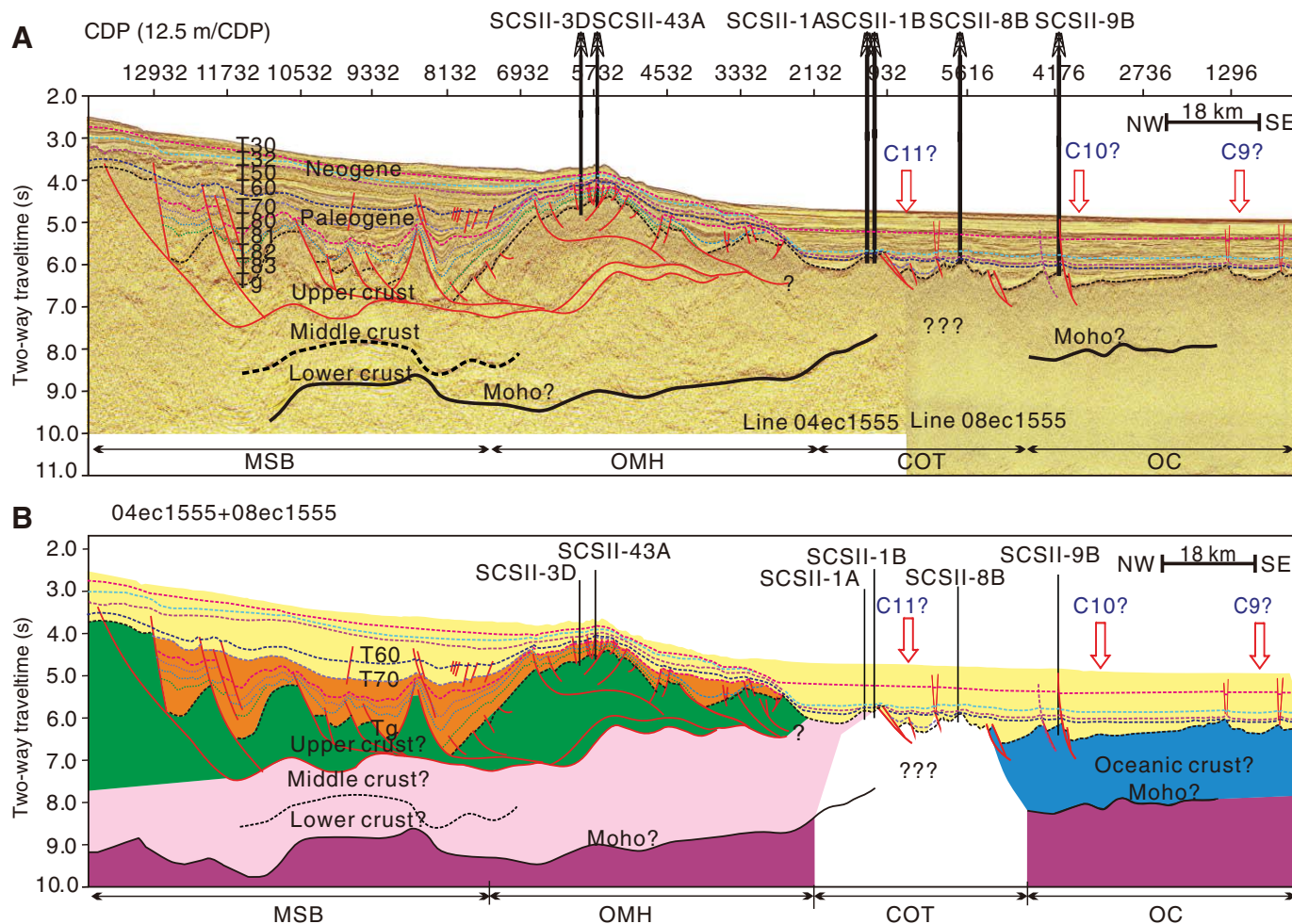
Figure F6. Simplified interpretation of seismic data shown in Figure F4. Note the seaward shallowing of the Mohorovicic seismic discontinuity (Moho) and presence of major detachment faults that seem to sole out between the upper and middle/lower crust. Although the general location of the continent-ocean transition (COT; white with question marks) is well constrained by both seismic profiles (Figures F3, F4), the details of crustal structure within the COT are not well constrained. The seismic line in Figure F5 images this zone slightly better, in particular regarding the Moho.
