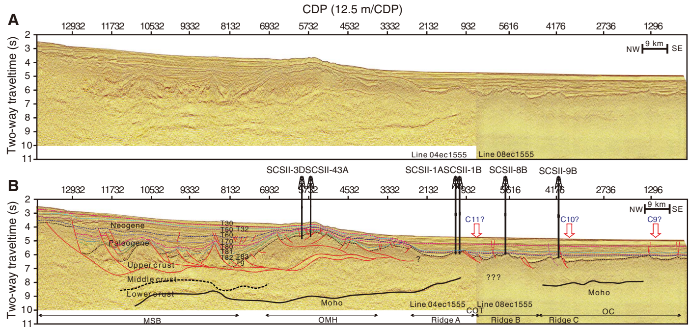
Figure F4. Deep crustal time-migrated seismic reflection data (A) without interpretation and (B) with interpretation. Note the rather thin lower crust (two layers) above a strong Mohorovicic seismic discontinuity (Moho) reflector that can be followed oceanward. Moho reflection is weak to absent seaward from around the interpreted continent–ocean transition (COT). Wide-angle seismic data (Yan et al., 2001) confirm ~6 km thick ocean-type crust to be present seaward of the COT. A large detachment fault ~150 km inland of the COT separates more stable crust landward from that of highly extended crust seaward. An outer margin high is a fairly consistent feature along this margin segment. Key seismic unconformities are shown in purple (T70; ~32 Ma breakup unconformity?) and blue (T60; ~23 Ma regional basin event). These ages are inferred from long distance (>100 km) correlation of seismic unconformities with industry holes and ODP Leg 184 Site 1148 (T60). These ages need confirmation by coring, and are only tentative. Tg unconformity (green) is basement. Approximate position of seafloor magnetic anomalies with chron numbers are shown by arrows. See Figure F6 for a schematic interpretation of the entire profile. Seismic data is from Line 04ec1555-08ec1555 (courtesy of the Chinese National Offshore Oil Corporation). Location of line is shown in Figure F2.
