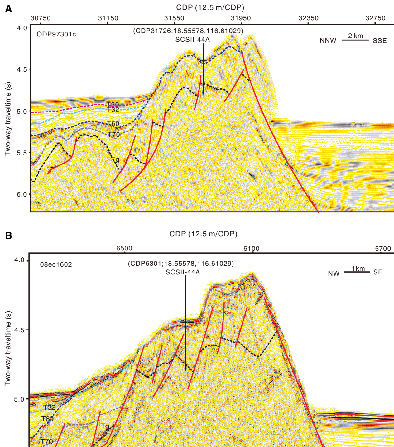
Figure AF9. (A) Primary seismic Line ODP97301c and (B) crossing Line 08ec1602, proposed Site SCSII-44A. CDP = common depth point. Dashed lines = unconformities, solid red lines = faults.
