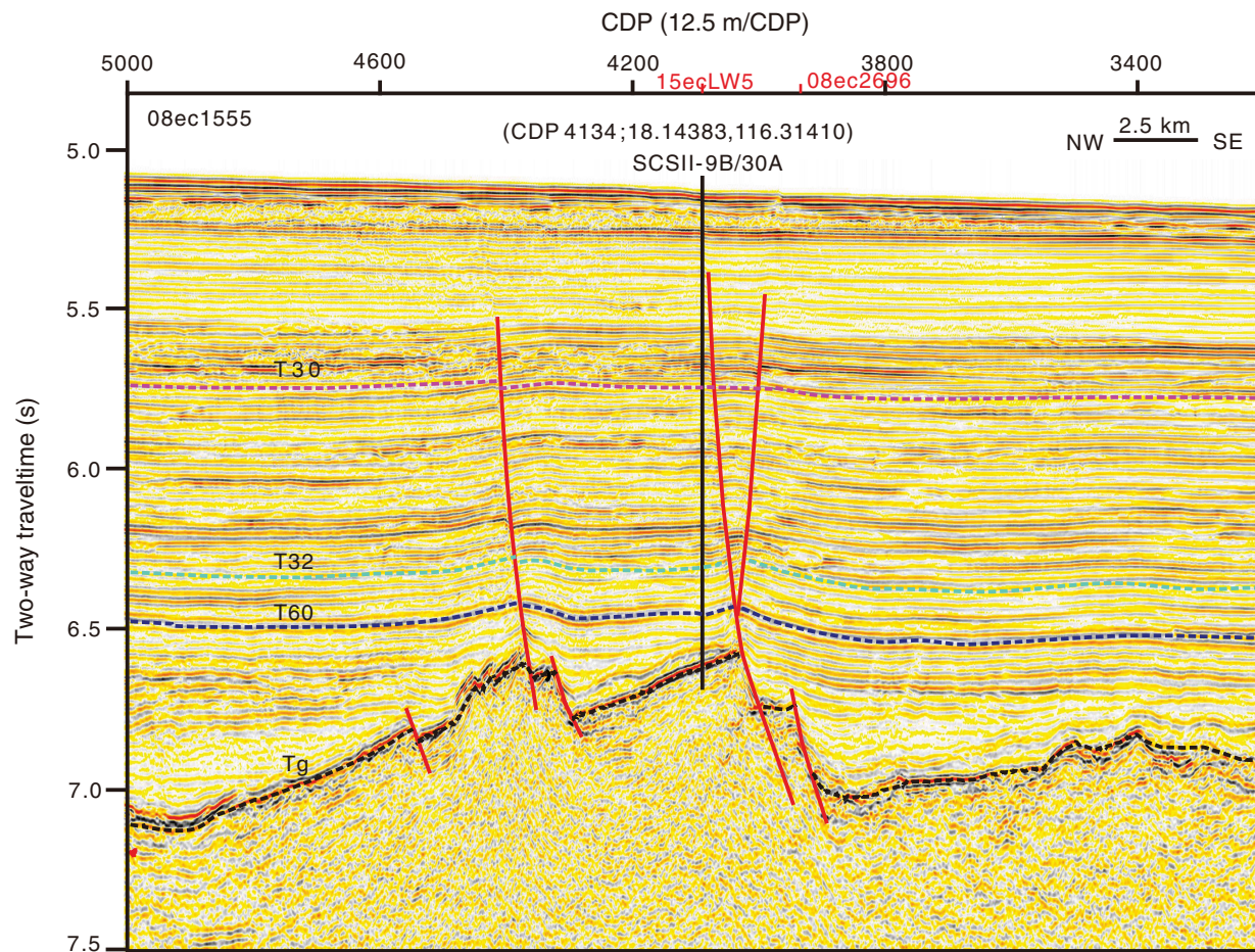
Figure AF28. Seismic Line 08ec1555. Primary seismic line for proposed Site SCSII-9B and crossing seismic line for proposed Site SCSII-30A. CDP = common depth point. Dashed lines = unconformities, solid red lines = faults.
