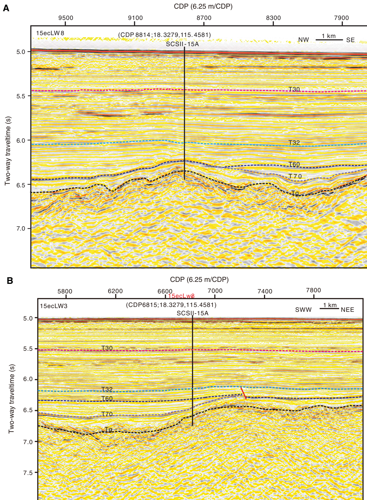
Figure AF15. (A) Primary seismic Line 15ecLW8 and (B) crossing Line 15ecLW3, proposed Site SCSII-15A. CDP = common depth point. Dashed lines = unconformities, solid red line = fault.
