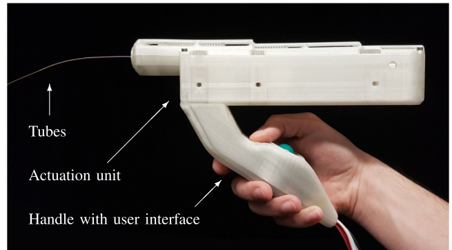
Fig. 1. Proposed hand-held concentric tube robot with deployed tubes, actuation unit, and handle equipped with a user interface.
