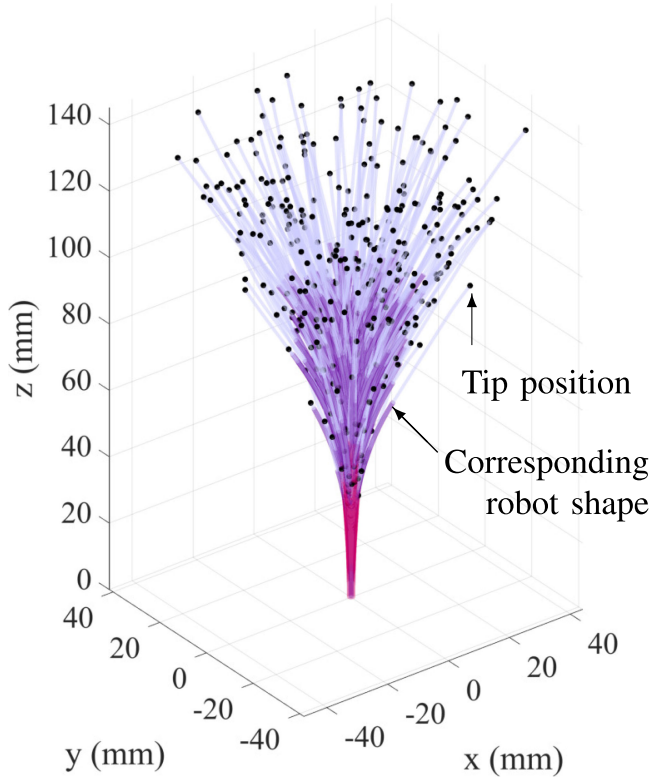
Fig. 8. Illustration of a set of random CTR configurations, with the tubes of each configuration represented in magenta, violet, and gray, and the corresponding tip positions highlighted in black.
