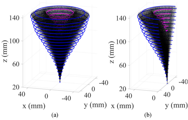
Fig. 14. Illustration of point cloud \mathcal{P} with the inner and outer boundaries of the workspace in magenta and blue, respectively. Boundaries are represented every 6 mm for each of visualization.
