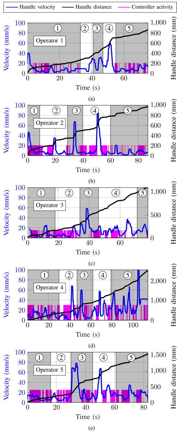
Fig. 21. Interaction between operators and the device over time while reaching targets 1–5, with plots (a)–(e) corresponding to operators 1–5. Magenta lines represent an interaction of the operator with the inputs on the device handle, while the blue lines represent the instantaneous velocity of the device handle and the black line its distance traveled by the handle over time.
