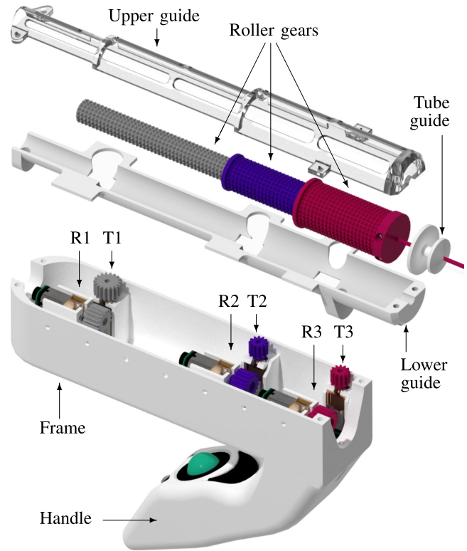
Fig. 4. Exploded view of the proposed hand-held CTR, with its main components. R1, R2, R3, T1, T2, and T3 designate the actuator and associated gear for the rotation and translation of tubes 1, 2, and 3, respectively.
