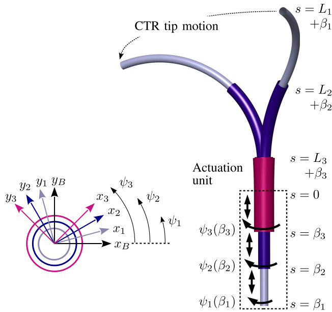
Fig. 2. On the right: illustration of a three-tube CTR with deployed tube lengths L_i + \beta_i and base angles \psi_i(\beta_i) . Two different configurations are represented, corresponding to different base angles of the tubes. On the left: cross-sectional view of the three overlapping tube link of the CTR, with the angle of the tubes relative to the Bishop frame.
