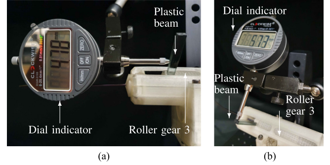
Fig. 15. (a) Illustration of backlash measurement for the translation of roller gear 3 (T3). (b) Illustration of backlash measurement for the rotation of roller gear 3 (R3).
