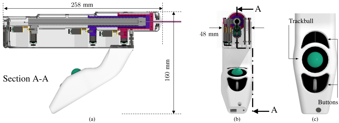
Fig. 5. (a) Cross-sectional and (b) back view of the prototype with its dimensions depicted, and (c) close-up view of the handle, including the user inputs. The frame and guides (upper and lower) are shown as transparent to enable visualization of the internal components.
