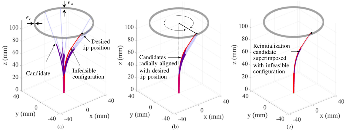
Fig. 9. Illustration of the search for a reference configuration in the case of 10 candidates in three steps. (a) Identification of reinitialization candidates. (b) Radial alignment of the reinitialization candidates' tip with the desired tip position. (c) Selection of reinitialization configuration.
