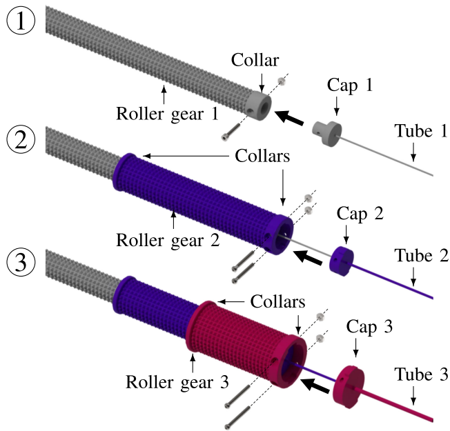
Fig. 3. Sequence of assembly steps (labeled from 1 to 3) for the attachment of the tubes, which are preassembled on their respective caps, to the roller gears. The final assembly is then inserted in the lower guide and covered by the upper guide as illustrated in Fig. 4.
