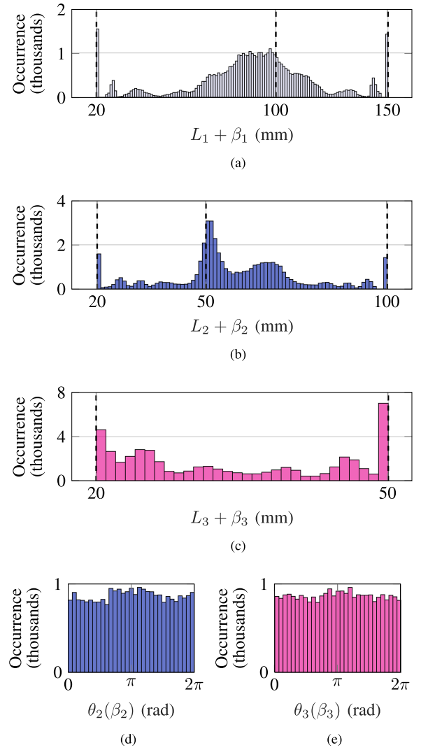
Fig. 13. Histograms showing the distribution of L_i + \beta_i (deployed length of tube i ) and \theta_i(\beta_i) (base angle of tube i relatively to tube 1) for all points of \mathcal{P} that have a position error greater than 0.3 mm.
