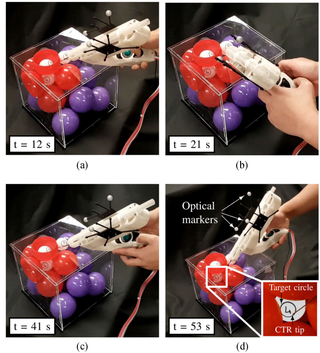
Fig. 20. Timelapse representing the pose of the device with respect to the environment of navigation for operator 2, with the images taken at (a) 12, (b) 21, (c) 41, and (d) 53 s. (d) contains a close-up view with the CTR tip reaching target 4.
