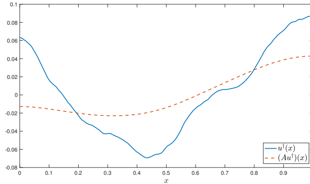
FIGURE 5.1. The true state u^\dagger used throughout Section 5.1, and its image Au^\dagger under the blurring operator A .
