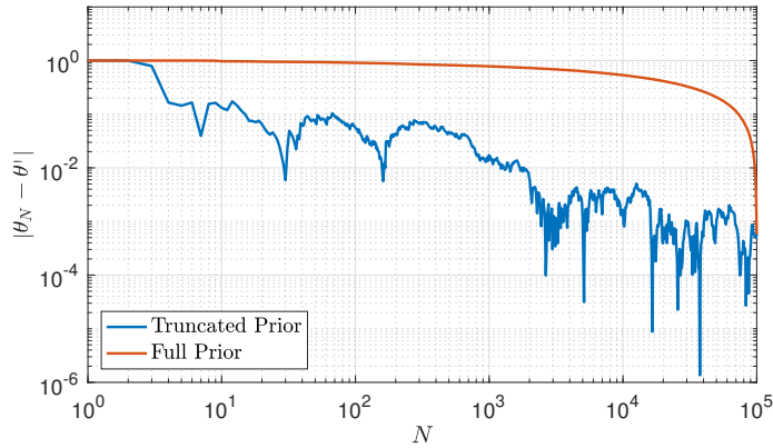
FIGURE 5.2. The trace of the errors between the minimizers of J_{\text{NC}}^{N,\gamma_N} and \widetilde{J_{\text{NC}}^{N,\gamma_N}} and the true hyperparameter, as defined in Section 5.2, as N is increased.
