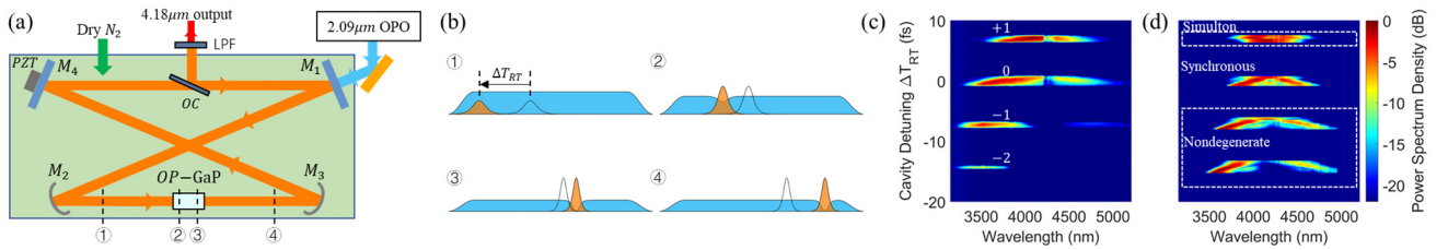
Fig. 1 (a) Schematic of the experimental setup. (b) Illustration of simulton formation: signal (orange) at \omega and pump (blue) at 2\omega . Solid lines (uncolored) denote a perfectly synchronous half-harmonic pulse undergoing linear propagation. \Delta T_{RT} denotes the delay with respect to the incoupled pump pulse that the signal pulse acquires due to the cavity round-trip time detuning. (c) Measured signal spectrum as a function of cavity detuning for 420 mW of \sim 50 -fs pump pulses, labeled with peak numbers. (d) Simulated signal spectrum as a function of cavity detuning, with the three identified regimes indicated.
