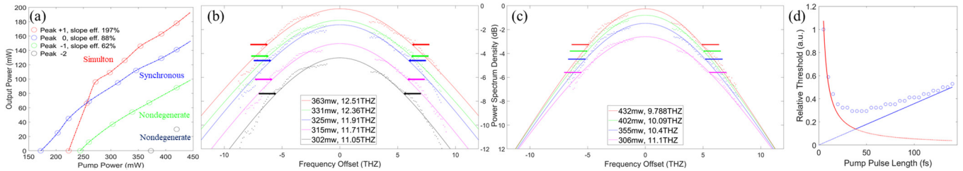
Fig. 2 (a) Measured output power for each peak (circles). Dashed curves are to guide the eye. (b), (c) Spectra recorded as a function of pump power for the 4.18- \mu\text{m} OPO working in simulton and synchronous regime, respectively. The corresponding pump power and FWHM bandwidth for each curve is denoted in the legend. The FWHM bandwidths are also denoted by colored arrows on the curves. (d) Simulated threshold dependence on pump pulse width for the simulton OPO at 4.18 \mu\text{m} (circles). Two asymptotes are plotted to show the tendencies based on a reduced OPO theory (solid curves).
