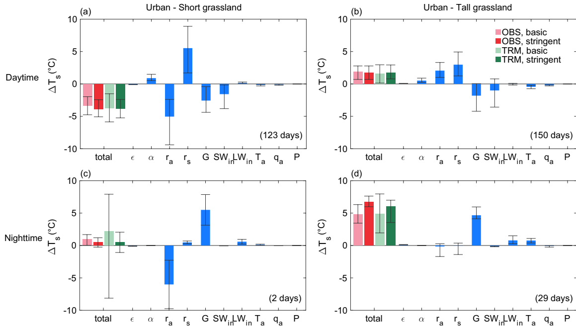
FIGURE 6 Attribution results of surface urban heat islands using the Two Resistance Mechanism (TRM) model during (a, b) daytime (10am-4pm) and (c, d) nighttime (10pm-4am). For (a, c), the short grassland site is used as the reference site, and for (b, d) the tall grassland site is used as the reference site. The sample size is noted in the bracket in the bottom right corner of each panel. The column indicates the median of the results at the daily scale, and the upper and lower error bars are the 80th and 20th percentiles of the results, separately, representing the day-to-day variability of the attribution results. “Basic” refers to applying the basic data filtering strategy, where we only exclude the half-hourly data when any one of the three sites have a missing value. “Stringent” refers to applying the more stringent data filtering strategy, where we further exclude the data when absolute value of the sensible heat flux or latent heat flux is small (less than 15 \text{ W m}^{-2} for daytime and 0.1 \text{ W m}^{-2} for nighttime) and when the inferred aerodynamic resistance or surface resistance is negative.
