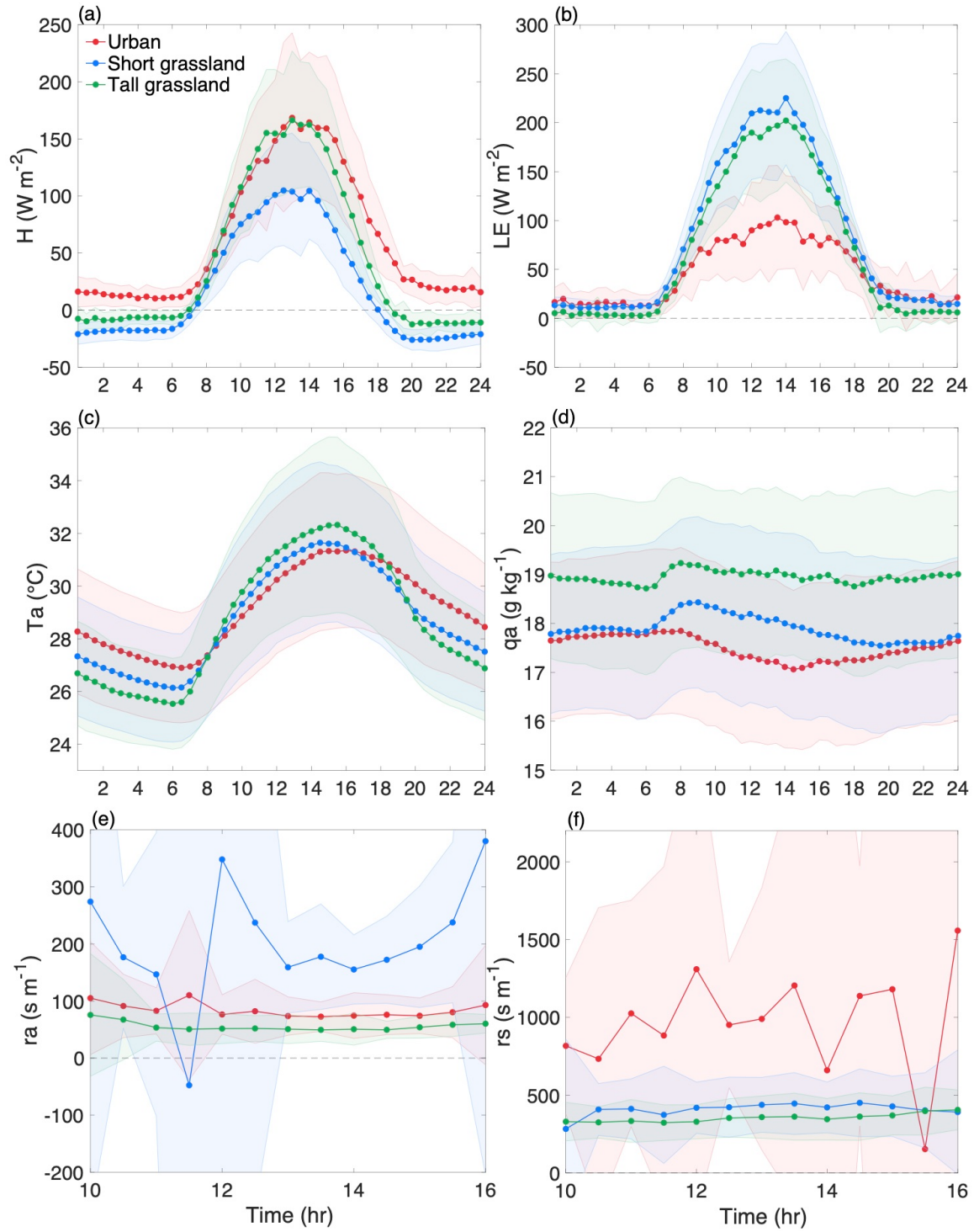
FIGURE 4 Average diurnal cycles of (a) sensible and (b) latent heat fluxes and their controlling factors, including (c) air temperature, (d) air specific humidity, (e) aerodynamic resistance and (f) surface resistance. For (e) and (f), only the daytime (10am to 4pm local time) results are shown. The shading denotes standard deviations.
