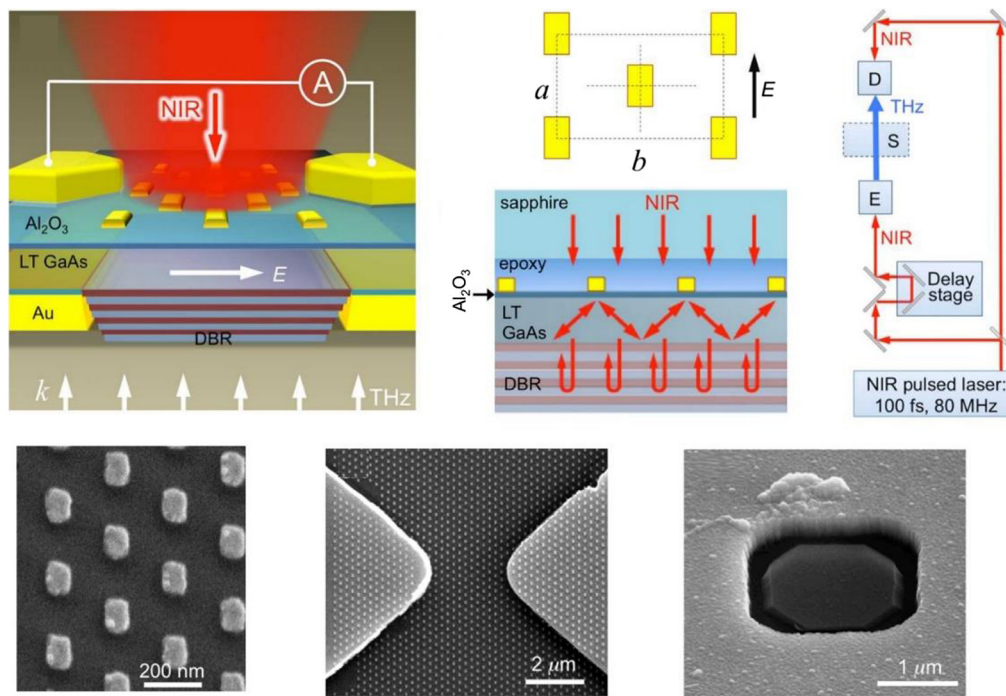
Fig. 13 Optical nanocavities and DBR. The SEM images left to right illustrate gold antenna array, the active region of the THz detector showing two metallic electrodes and the nanoantenna array in the PC gap; a 2- \mu\text{m} square input aperture in the gold screen of the near-field THz probe. Figure retrieved from Ref. 177 with permission from the American Chemical Society.
