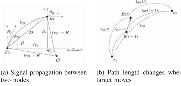
Fig. 2: Signal propagation path length in isogradient acoustic signal speed sea water
