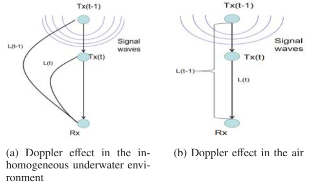
Fig. 1: Doppler effect when transmitter moves down to the receiver at a constant speed
