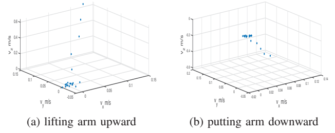
Fig. 4: VTb estimation results using dynamic self-refining optimization and underwater DFS coefficients
