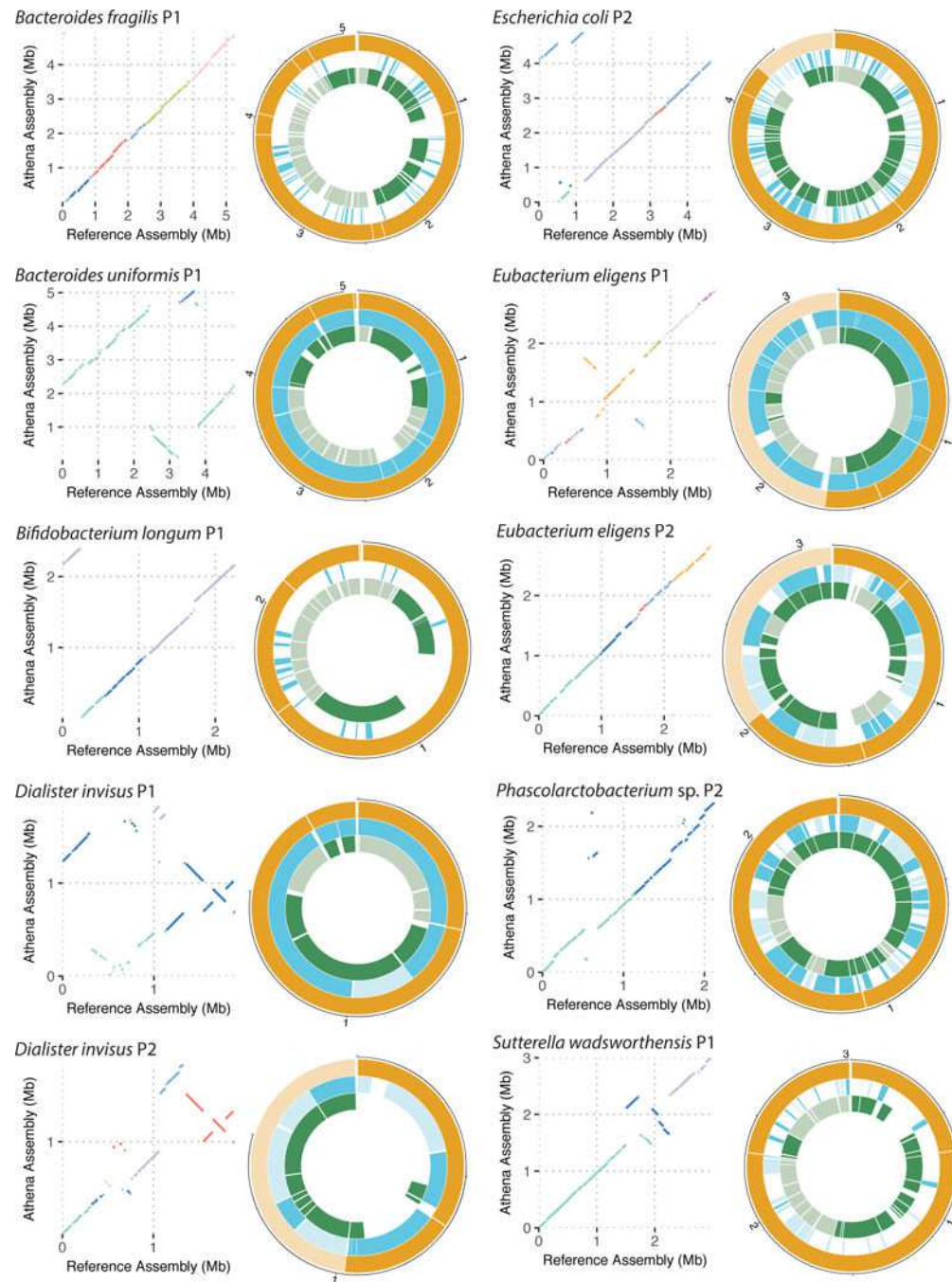
Figure 5. Comparisons of representative read cloud genome drafts to reference genomes, and corresponding short read and SLR drafts. Dot-plot alignments between read cloud drafts (y-axis) and the closest available reference genome (x-axis) are shown. For each dot-plot, a given color corresponds to the alignment of a single contig in the read cloud draft against the available reference. Large-scale structural concordance and also differences including inversions are visually apparent. Alignments of SLR and short read drafts to the read cloud drafts for each taxon are also shown. In all cases, read cloud drafts were the most contiguous. For each approach, contigs belonging to the
