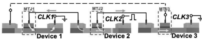
Fig. 3. Schematic of DW-MTJ based shift register.
