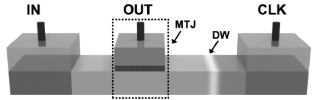
Fig. 1. Device diagram of DW-MTJ.
