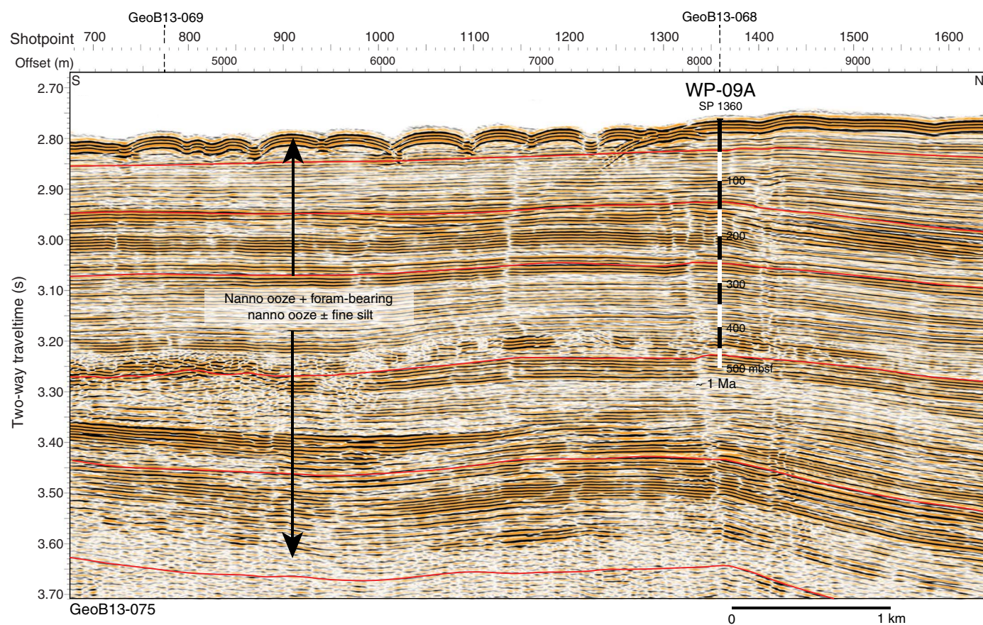
Figure AF10. Seismic reflection profile Line GeoB13-075 with location of proposed Site WP-09A (6°20.81'N, 125°50.89'E; shotpoint [SP] 1360; water depth = 2080 m; target depth = 350 mbsf; approved depth = 500 mbsf). Locations of crossing seismic profile lines shown with dashed lines at top. Red dashed lines trace reflectors.
