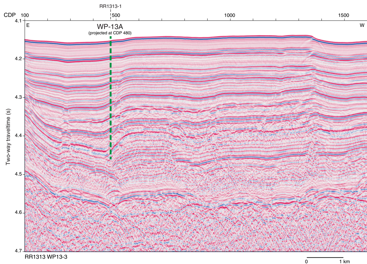
Figure AF14. Seismic reflection profile Line RR1313 WP13-3 with location of alternate proposed Site WP-13A ( 16^{\circ}3.98'N , 124^{\circ}42.03'E ; projected at common depth point [CDP] 480; water depth = 3077 m; target depth = 280 mbsf; approved depth = 280 mbsf) projected 2.9 km south onto the line. Locations of crossing seismic profile lines shown with dashed lines at top.
