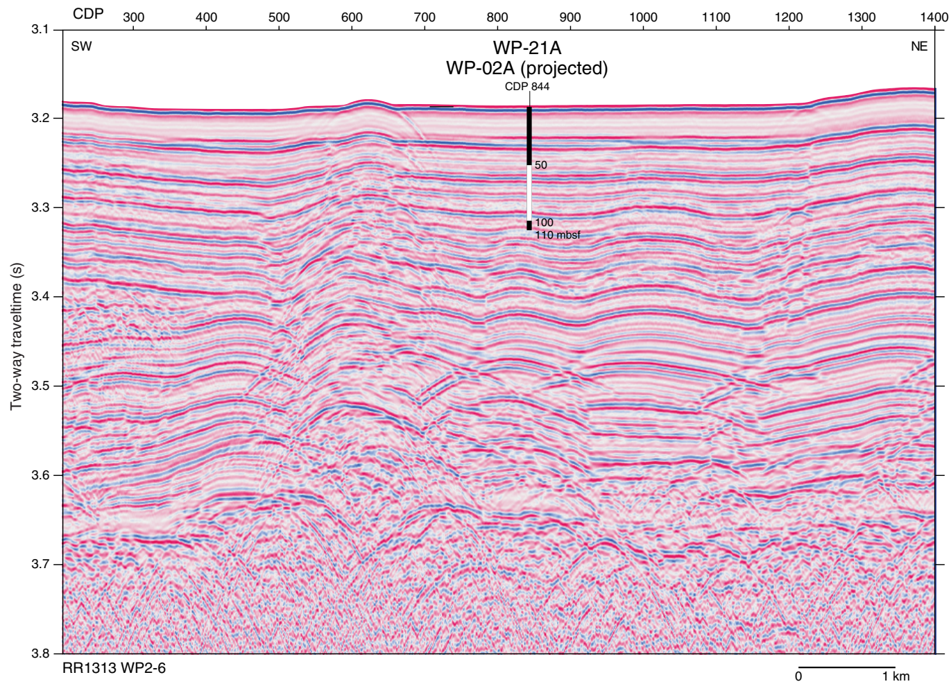
Figure AF32. Seismic reflection profile Line RR1313 WP2-6 with location of alternate proposed Site WP-21A ( 5^{\circ}49.59'N , 142^{\circ}37.33'E ; common depth point [CDP] 844; water depth = 2355 m; target depth = 100 mbsf; approved depth = 150 mbsf) and proposed Site WP-02A ( 5^{\circ}48.95'N , 142^{\circ}39.26'E ; CDP 844; water depth = 2355 m; target depth = 250 mbsf; approved depth = 430 mbsf) projected 3.6 km west onto the line. Location of crossing seismic profile line shown with dashed line at top.
