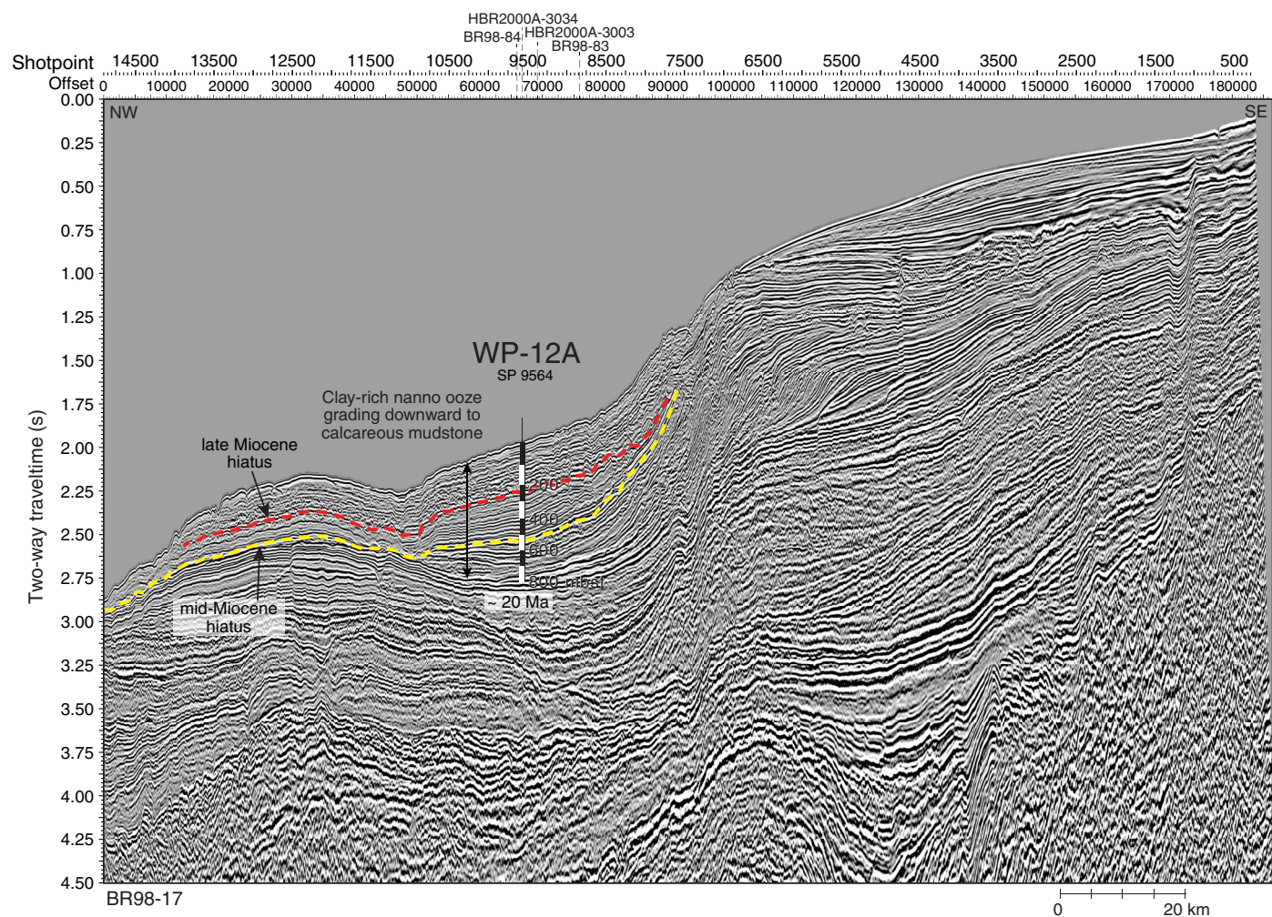
Figure AF4. Seismic reflection profile Line BR98-17 with location of alternate proposed Site WP-12A (15°5.646'S, 120°25.74'E; shotpoint [SP] 9564; water depth = 1480 m; target depth = 500 mbsf; approved depth = 800 mbsf). Locations of crossing seismic profile lines shown with dashed lines at top. Red dashed line = inferred late Miocene hiatus; yellow dashed line = inferred mid-Miocene hiatus.
