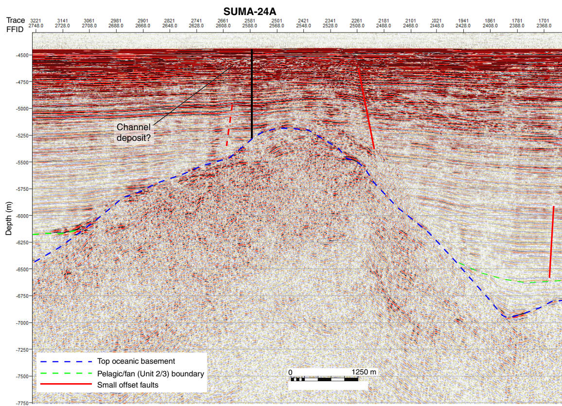
Figure F6. Interpreted seismic Profile WB10 in the vicinity of proposed Site SUMA-24A (S. Singh, unpubl. data; vertical exaggeration = 2). Depth-migrated section (with interpretation: red = minor sedimentary faults, green dashed line = Unit 2/3 boundary [pelagic sediments to Nicobar fan sediments]), example buried channels, and top of basement also indicated.
