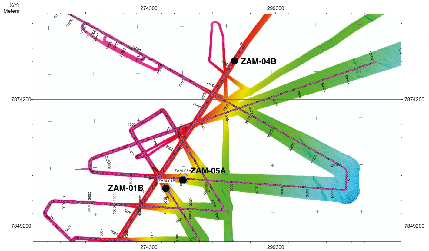
Figure AF5. Seismic line tracks with the bathymetry along the tracks showing Sites ZAM-01B, ZAM-04B, and ZAM-05A.
