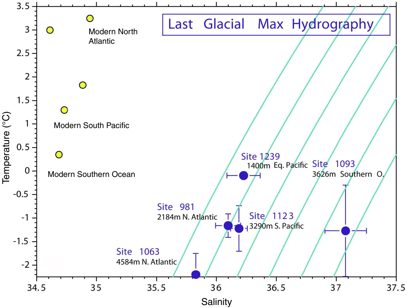
Figure F4. T-S plot for the LGM. Based on the type of pore water data we propose to collect here, this plot shows several differences with the modern. Yellow dots are the location of modern bottom waters where the cores for the blue LGM points were collected. The ODP site numbers and green isopycnals provide context.
