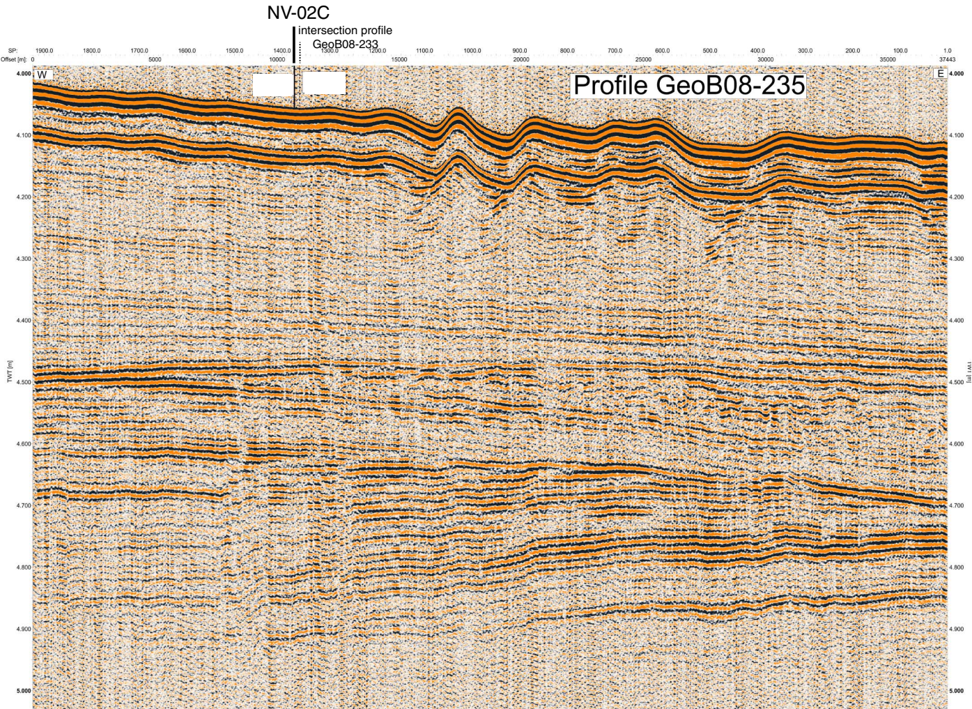
Figure AF14. Seismic Line GeoB08-235 with location of Site NV-02C.
