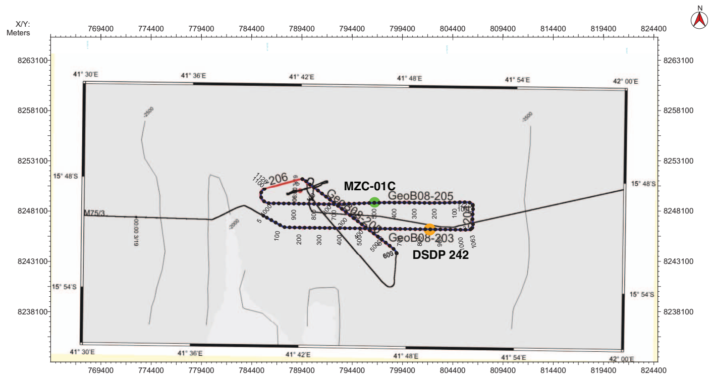
Figure AF1. Seismic line track map with the locations of Site MZC-01C and DSDP Site 242. Contour lines = bathymetry.
