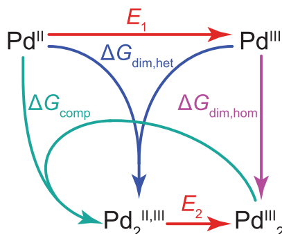
Scheme 1. Summary of the Reactions between Pd II , Pd III , Pd III , and Pd 2 II,III
