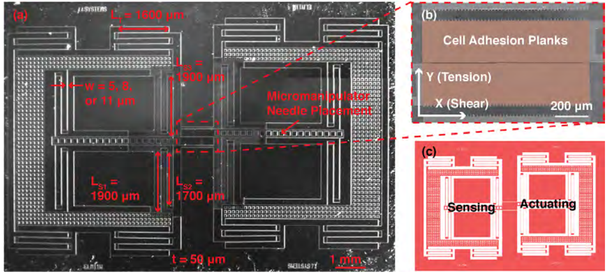
Figure 1. Folded flexures placed in parallel suspend the cell adhesion planks of the cell mechanics device. (a) The silicon die ( 8.5 \times 12.4 mm) features two cell culture regions or ‘planks,’ each suspended by four symmetric sets of folded flexures to provide compliance in Y, and another four sets to provide compliance in X. The Y (tension) stiffness of the device is defined by dimensions ( L_T , w , and t ) of the tension beams, and the X (shear) stiffness of the device is defined by dimensions ( L_{S1} , L_{S2} , L_{S3} , w , and t ) of the shear beams ( L : Length, w : width, t : thickness). (b) These flexures enable relative motion of the planks to apply tension or shear to an adhered cell monolayer, where the force across the monolayer may be calculated based on the spring stiffness in each direction. (c) All of the moving components (actuating and sensing) of the device are defined by a single lithographic mask.
