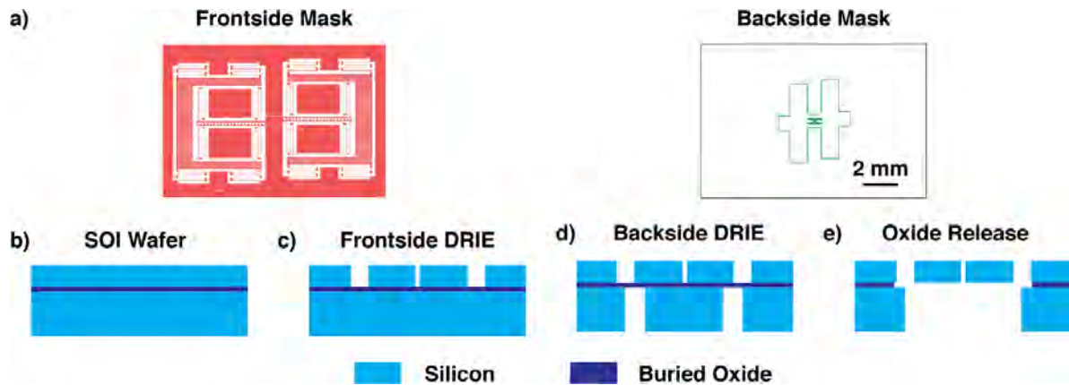
Figure 2. The devices are defined by two lithography steps, and frontside and backside DRIE. (a) Frontside etch mask layout and backside etch mask layout. (b) Anneal SOI to release built-in stress in the buried oxide. (c) Define frontside structures using a DRIE process. (d) Define backside release areas under moving structures and flexures using a DRIE process. (e) Release the moving structures by etching the BOX in BOE.
