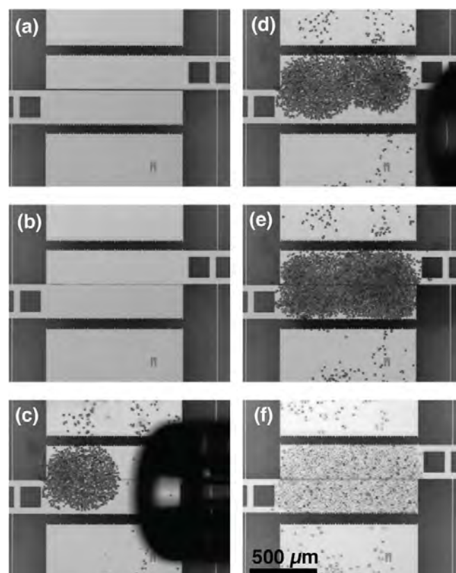
Figure 4. Placing a controlled cell population enables reproducible experiments and minimizes potential for interference in the flexure regions. (a–b) The actuation plank (top) is moved 5\ \mu\text{m} in tension to close the gap to the sensing plank (bottom). (c–e) E-cadherin:dsRed MDCK cells are delivered in three steps ( \sim 900 cells each) using a micro-capillary tube. (f) MDCK cells form a monolayer across both planks 3 h after cell seeding.
