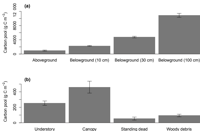
Figure 2. Average carbon density of all sites in the Y4 watershed (a: above- and belowground to 1 m; b: aboveground only). Bars indicate standard error.
