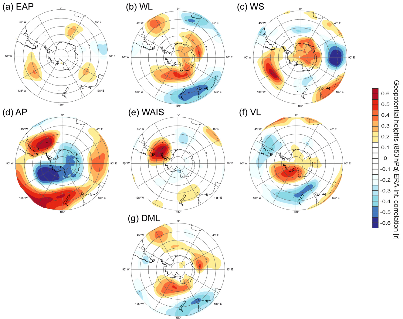
Figure 4. Spatial correlation plots of standardized regional snow accumulation composites with annual 850 hPa geopotential heights from ERA-Interim (1979–2010). Grid points with > 95 % significance are dotted. Note that correlation with WS only covers the period 1979–1992.
