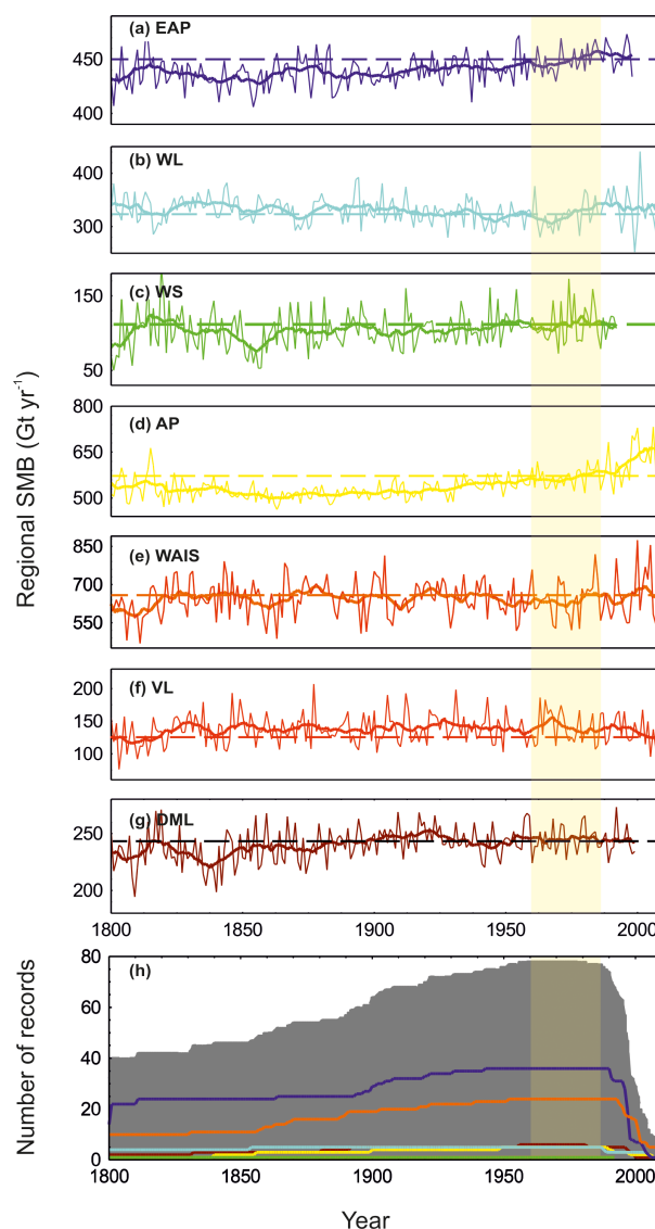
Figure 6. Regional SMB composites (1800–2010 AD) shown as annual averages (thin lines) and 5-year means (thick lines) for (a–g) the East Antarctic Plateau (EAP, dark blue); Wilkes Land coast (WL, cyan), Weddell Sea coast (WS, green), Antarctic Peninsula (AP, yellow), West Antarctic Ice Sheet (WAIS, orange), Victoria Land (VL, red), and Dronning Maud Land (DML, brown). Panel (h) represents the total number of records (solid grey) and the number of records by region.
