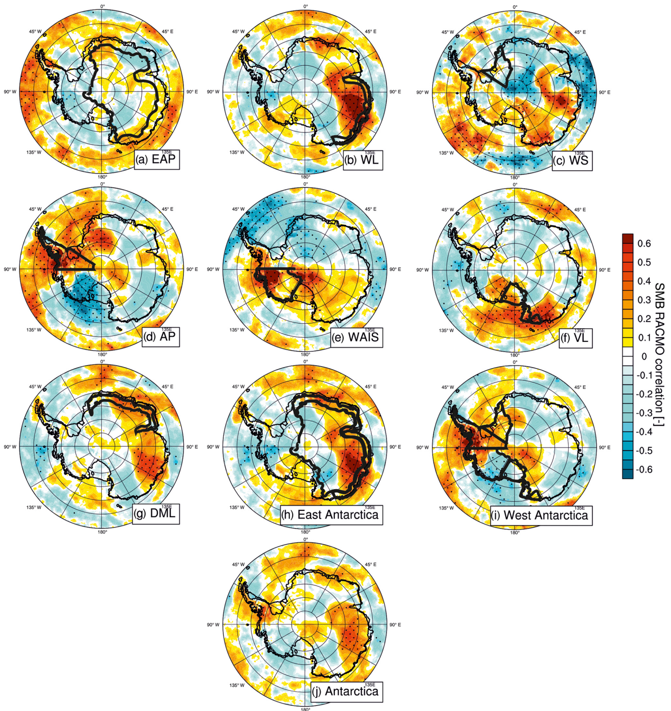
Figure 2. Spatial correlation plots of standardized regional and continental composites of snow accumulation with SMB from RACMO2.3p2 (1979–2010). Grid points with >95 % significance are dotted. Note that correlation with WS only covers the period 1979–1992.
