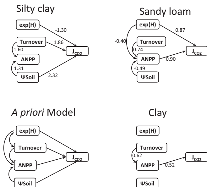
Fig. 4. Structural equation models relating the CO 2 responses of 0- to 40-cm soil water potential (Ψ soil ), aboveground net primary productivity (ANPP), turnover in community composition, and effective species richness, exp(H), to the CO 2 response of soil CO 2 efflux, J CO2 . The a priori model was fit separately to the individual soil series. Depicted paths indicate significant direct effects. Nonsignificant paths are omitted in the fitted models. See Table 3 for model fit statistics, Fig. 5 for visualization of total effects, and SI Appendix, Table S3 for partitioning of direct and indirect effects.
