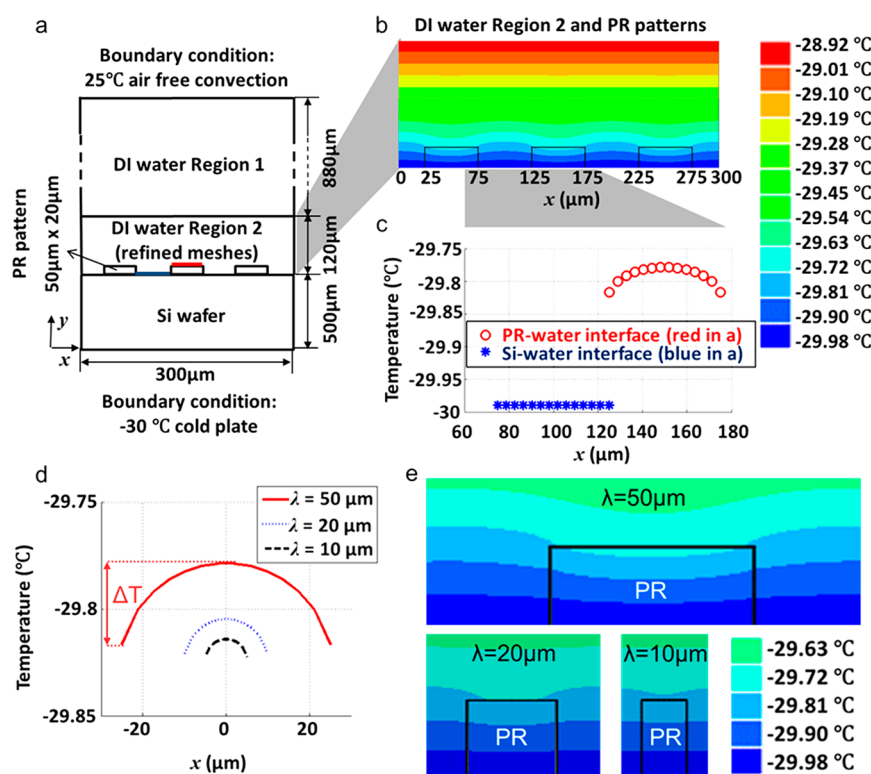
Figure 2. (a) The sketch, dimensions, and boundary conditions of a 2D model for FEA simulation. (b) The 2D temperature profile in the neighborhood of Si, PR, and DI interfaces. (c) The temperature curves of PR–water interface and Si–water interface. (d) Temperature curves of PR–water interface with various \lambda values. (e) 2D temperature profiles in the neighborhood of PR patterns with varying \lambda values.
