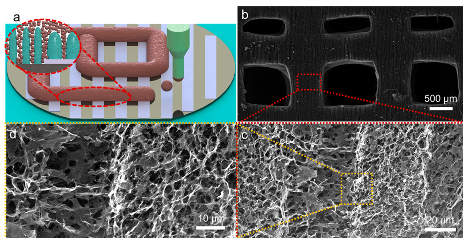
Figure 5. (a) Schematics of the 3D freeze printing process using substrates with patterned PR features. (b–d) Low and high-magnification SEM images showing the tailored microstructure of the graphene oxide aerogels fabricated through the 3D freeze printing process using the patterned Si substrate with \lambda = 48.64\text{ }\mu\text{m} .
