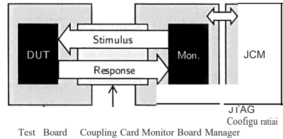
Fig. 4. Test setup.
