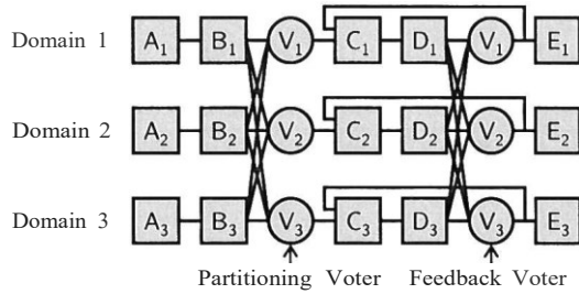
Fig. 2. Diagram of full TMR with partitioning and feedback voters.
