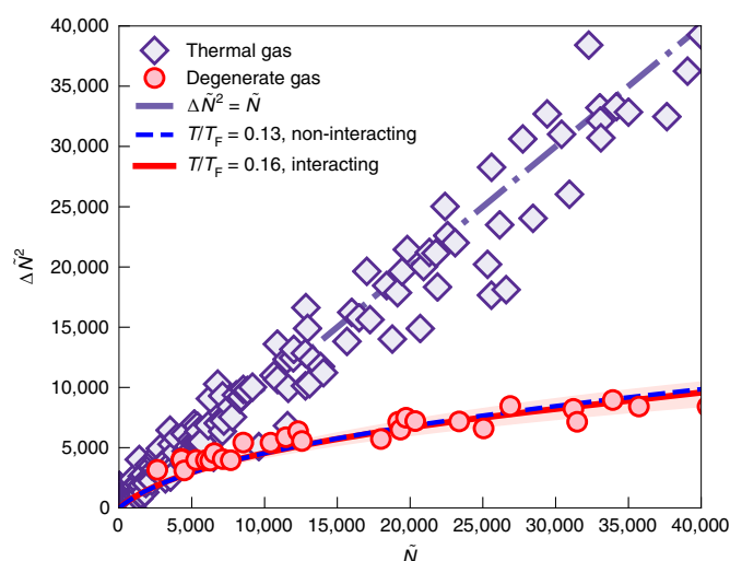
Fig. 3 | Local density fluctuations of an SU( N ) degenerate gas. Density fluctuations after 11.5 ms time of flight for a degenerate cloud with N=10 nuclear spin states. The data are fitted using an SU( N ) interacting model to extract T/T_F=0.16 , with shading representing a 2\sigma uncertainty of \pm 0.02 T/T_F . Fitting the data instead to a non-interacting ideal Fermi gas gives T/T_F=0.13 , showing an interaction-induced suppression of \sim 20\% . The difference between the interacting and non-interacting fits is much less than the scatter in the data, highlighting the indistinguishability between interacting and non-interacting systems when measuring density fluctuations alone at the given signal-to-noise ratio. The total density fluctuations are 25% of that of the thermal gas. A thermal cloud reproduces Poisson statistics with \Delta\tilde{N}^2/\tilde{N}=1 . Each data point is obtained by looking at the atom number variation and mean in a subregion of the cloud for a series of images.
