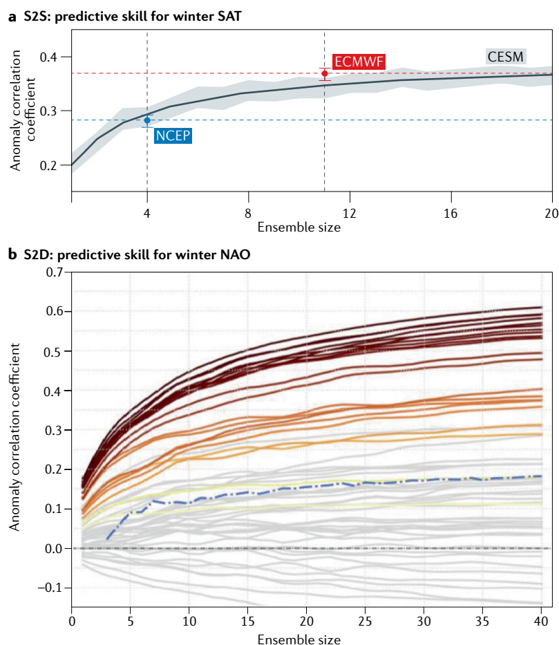
Fig. 2 | Influence of ensemble size and lead year ranges on predictive skill. a | Skill (as measured by the anomaly correlation coefficient (ACC)) in predicting subseasonal to seasonal (S2S) globally averaged NDJFM surface air temperature (SAT) (excluding the Antarctic) from CESM initialized hindcasts of various ensemble size (grey line). Shading denotes the 5% and 95% significance levels. Blue and red whiskers illustrate predictive skill for NCEP Climate Forecast System version 2 (CFSv2) and ECMWF subseasonal hindcasts, respectively. b | Skill (as measured by the anomaly correlation coefficient) in predicting seasonal to decadal (S2D) wintertime North Atlantic Oscillation (NAO) using ensembles of different sizes from the Decadal Prediction Large Ensemble (DPLE) 20 . Each line depicts a different lead year range, with those that are coloured corresponding to statistically significant correlations; the darker the shading, the greater the statistical significance. Dashed-dotted line shows the skill of the sub-ensemble mean against a single member of the ensemble (averaged for all possible combinations). Both panels illustrate that the more ensemble members, the higher the skill for longer lead year ranges. Panel b is adapted from REF. 37 , CC BY 4.0 ( https://creativecommons.org/licenses/by/4.0/ ).
