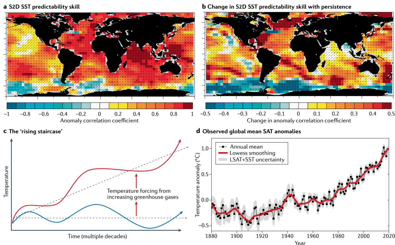
Fig. 6 | S2D predictions and aspects of time-evolving globally averaged temperature. a | Prediction skill, measured as the anomaly correlation coefficient, of sea surface temperature (SST) averaged over lead years 5–9 from the Decadal Prediction Large Ensemble (DPLE) 20 ; darker red indicates higher skill. b | Improvement in prediction skill from initialized predictions in panel a over and above a persistence prediction; darker red indicates better skill in the initialized predictions, thus showing the value-added of initialized predictions. c | Schematic of the ‘rising staircase’, illustrating how natural decadal-scale temperature fluctuations (blue) are tilted upwards owing to anthropogenic greenhouse gas emissions (red), producing accelerated warming in some decades and reduced warming in others. d | Time series of observed global mean surface air temperature (SAT) anomalies (land surface air temperature (LSAT) and sea surface temperature (SST)) showing characteristics of the rising staircase: accelerated warming over 1980–2000 and 2014–present, and a slowdown in the rate of warming over 2000–2014. S2D, seasonal to decadal. Panels a and b adapted from REF. 20 © American Meteorological Society. Used with permission. Panel c adapted with permission from National Academies Press, from REF. 267 ; permission conveyed through Copyright Clearance Center Inc. Panel d adapted, with permission, from REFS 270,271 , NASA.
