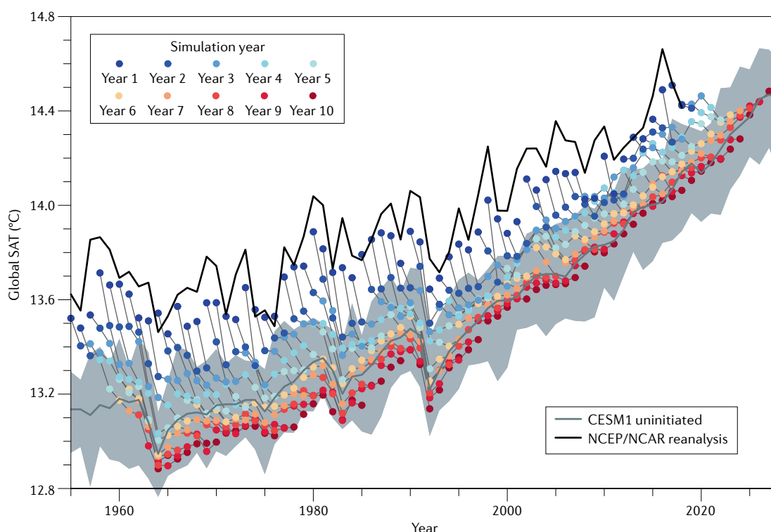
Fig. 4 | Impact of model drift on initialized predictions. Globally averaged surface air temperature (SAT) predictions from the Decadal Prediction Large Ensemble (DPLE) 20 as a function of simulation year. Initial state predictions (blue dots) compare well with observations (black line), but drift (progression of blue dots to red dots) towards the model's systematic error state represented by the uninitialized state (dark grey line; grey shading is range of uninitialized projections).
