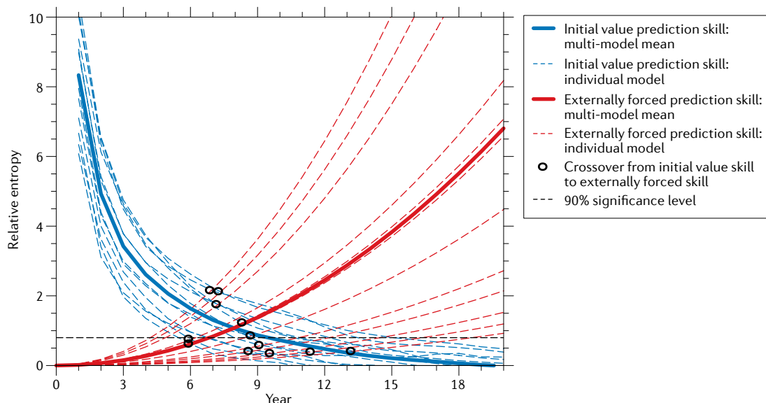
Fig. 1 | Timescales and processes involved with initialized predictions. a | Timescales and sources of predictability for subseasonal to seasonal (S2S), seasonal to interannual (S2I) and seasonal to decadal (S2D) timescales. Lighter green shading indicates larger uncertainty. b | Skill in predicting the upper 300 m of the Atlantic Ocean temperature, as measured by relative entropy, in initialized models (blue) and those forced by RCP4.5 (red). Skill is high for initialized predictions on S2S and S2I timescales (<2 years), but decreases towards S2D (years 3–9), after which time the skill from external forcing increases. AMV, Atlantic multi-decadal variability; ENSO, El Niño–Southern Oscillation; GHG, greenhouse gas; GMST, global mean surface temperature; MJO, Madden–Julian Oscillation; NAO, North Atlantic Oscillation; PDV, Pacific decadal variability; QBO, Quasi-Biennial Oscillation; SSW, sudden stratospheric warming. Panel b adapted with permission from REF. 10 , Wiley ©2012. American Geophysical Union. All Rights Reserved.
