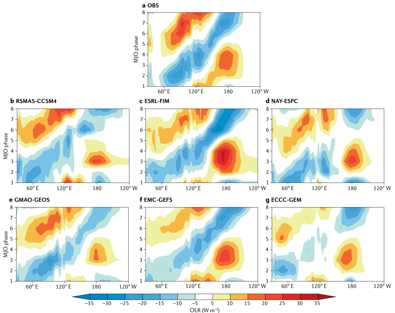
Fig. 5 | Initialized S2S predictions of the MJO. a | Observed outgoing long-wave radiation (OLR) anomalies averaged over 5° S–5° N as a function of the stage of the Madden–Julian Oscillation (MJO). b–g | As panel a but for various initialized predictions, with OLR anomalies taken as the average of simulations days 15–21. MJO events are identified based on Real-time Multivariate MJO (RMM) index amplitude \geq 1 . Eastward propagation of MJO-related OLR anomalies is well captured by all six models. S2S, subseasonal to seasonal. Adapted from REF. 6 , © American Meteorological Society. Used with permission.
