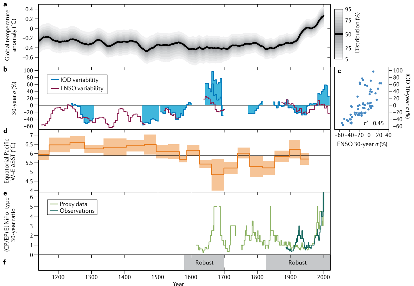
Fig. 3 | Extending proxy observations of S2D variability back in time derived from corals. a | Global mean surface temperature anomalies. b | 30-year running mean standard deviations of the coral-based Indian Ocean Dipole (IOD) (blue) and El Niño–Southern Oscillation (ENSO) (red). c | Scatter plot of the 30-year running mean standard deviations of coral-based IOD and ENSO. d | Equatorial Pacific west–east (W–E) sea surface temperature (SST) gradient (shading represents uncertainty). e | Central and eastern Pacific (CP/EP) El Niño derived from teleconnected climate patterns. f | An indication of reconstructions considered robust in panel e . Collectively, the panels illustrate a strengthening of IOD–ENSO decadal variability after ~1590. S2D, seasonal to decadal. Adapted with permission from REF. 58 , Springer Nature Limited.
