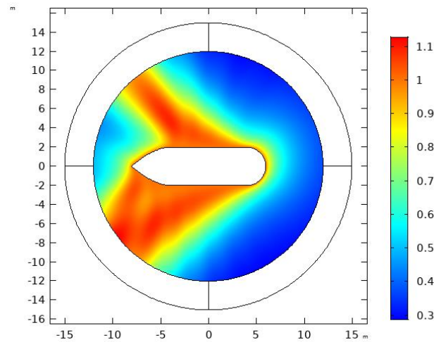
Fig. 4. Reflected electric field (V/m) from an incident plane wave
