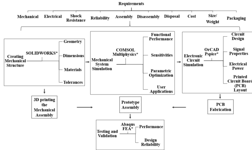
Fig. 1. Electro-mechanical assembly design process and key software platforms
