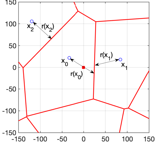
Fig. 7. An illustration of the JSP model with cell-dependent shadowing. Blue circles are BS locations generated from a PPP with \lambda = 3.5 \times 10^{-5} . Red lines are the Voronoi tessellation. The typical user denoted by the red square is located at the origin. r(x_i) is the length of the black line segment, which is the cell radius of x_i oriented towards the typical user.
