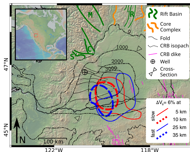
Figure 1. Map showing features that correlate with the central Columbia Basin downwarp. Accumulated thickness of the Columbia River Basalt (CRB) flows is indicated with black dashed lines (thickness in meters). CRB ponded in the downwarp, which subsided during the CRB eruptions. Subsidence centered on an Eocene rift basin associated with coeval core complex and trans-tensional basin activity in northern Washington State, USA. The Swauk (S), Chiwaukum (C), Republic (R), and Methow (M) grabens are labeled. The rift basin is imaged with active-source seismology along the cross section (indicated with triangles) (Catchings and Mooney, 1988; Fig. 2) and in three dimensions using surface waves (Gao et al., 2011). The anomalous crustal structure imaged in the immediate vicinity of the downwarp includes 5–6 km of sediment beneath ~4 km of CRB, and ~16 km of high-velocity lowermost crust interpreted by Catchings and Mooney (1988) to be rift-related magmatic underplate. Red and blue lines outline areas of low- and high-velocity crust (Gao et al., 2011). Topography adapted from Global Multi-Resolution Topography (GMRT) synthesis (Ryan et al., 2009).
