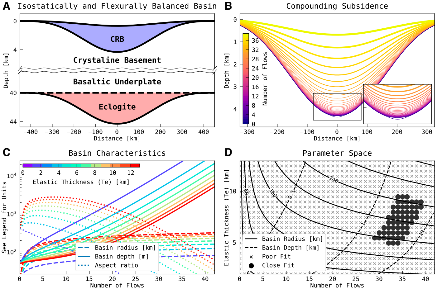
Figure 3. Models of time-evolving eclogite loading on an isostatically supported elastic plate. A: Beginning with a small depocenter, a larger basin develops by repeatedly filling the existing topography and modeling new subsidence owing to lower-crustal eclogite formation. B: Depositional interfaces over time, illustrating the compounding effect of the eclogitization subsidence mechanism. Each flow is deposited as a flat layer filling the previous depression, and subsequently downwarps as a result of newly generated eclogite. Color represents the sequence of deposition. Line thickness is proportional to the thickness of the basalt layer. Inset shows zoom-in of initial topography. C: Basin geometry characteristics over time, for varying elastic plate thicknesses. Other parameters are held constant across models. Basin depth increases slowly at first, and accelerates as the basin size, and hence load, increases. Basin radius rapidly adjusts to reflect the plate's natural flexural wavelength. Aspect ratio (radius/depth) reveals that, in this adjustment stage, radial growth briefly out-paces deepening. Long-term basin growth is dominated by deepening. D: The effects demonstrated in C trade off differently for different elastic plate thicknesses. Contours denote basin depth and radius over time for different plate thicknesses. Models whose geometries are similar to the Columbia Basin are plotted in filled circles, setting narrow limits on possible Miocene plate thickness.
