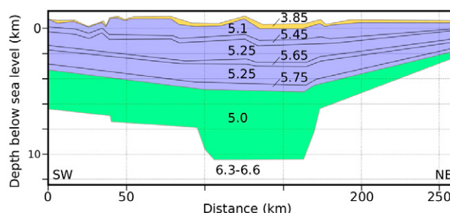
Figure 2. The upper crust along the cross section indicated in Figure 1 (after Catchings and Mooney, 1988). Numbers on plot give the P-wave velocity in km/s. Tan color is post-Columbia River Basalt (CRB) sediment; blue is CRB flows; green is Eocene sediment; white is basement. Note the deep sediment-filled rift basin, and CRB flows thickening toward the basin center, indicating that the basin subsided during deposition, and not after.
