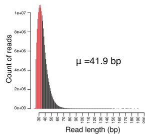
Extended Data Fig. 3 | DNA-fragment length distributions for nine mammoths. Reads are aligned to the LoxAfr4 autosomes. For the three Early and Middle Pleistocene samples (Krestovka, Adycha and Chukochya), reads of 25–200-bp length are shown; 30–200-bp reads are shown for the remaining
