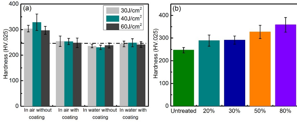
Fig. 2. (a) Surface hardness measurements under different processing conditions with laser fluence 30, 40 and 60 J/cm², the dash dot line represents the surface hardness of untreated material and (b) Surface hardness measurements for 20%, 30%, 50% and 80% overlapping ratio. The sample was treated with 40 J/cm² in air without coating.
