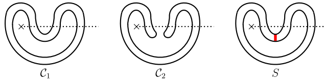
FIGURE 13. The saddle S: \mathcal{C}_1 \rightarrow \mathcal{C}_2 in Example 2.14.
