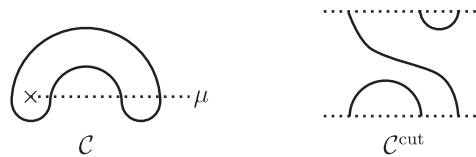
FIGURE 8. Cutting open a configuration \mathcal{C} along \mu to obtain a (3,3) -tangle \mathcal{C}^{\text{cut}} .
