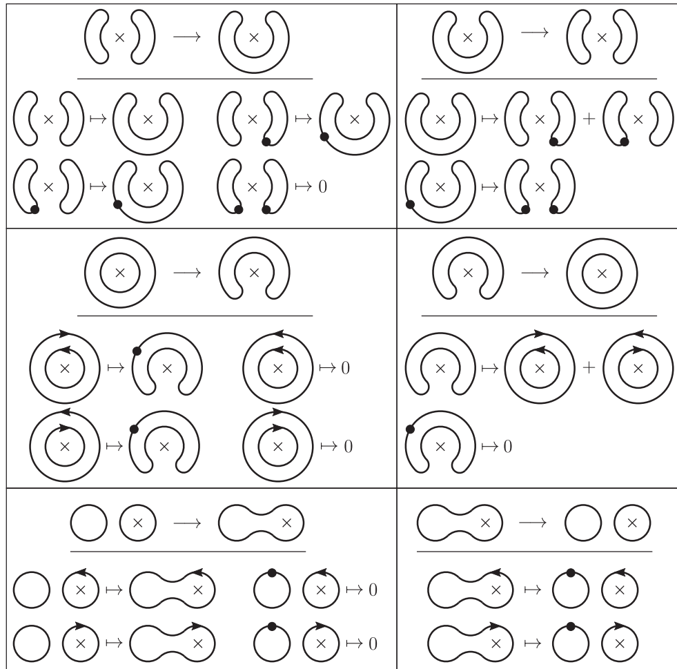
FIGURE 4. Surgery formulas in classical annular Khovanov homology. The table lists topological types of surgeries and corresponding maps on generators.
