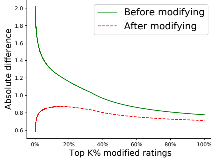
(a) Distance between the identified rating and average rating
