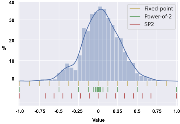
Fig. 1. Quantization levels by fixed-point, power-of-2, and SP2 in 4-bit weight representation precision, and weight probability distribution of the 4th layer in MobileNet-V2.
