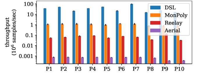
Fig. 15. Timescales benchm.: DSL, MonPoly, Reelay, Aerial.
