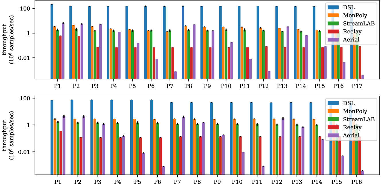
Fig. 13. Past-time microbenchmark: DSL, Reelay, MonPoly, Aerial.
