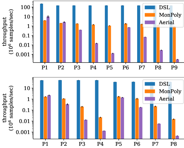
Fig. 14. Future-time microbenchmark: DSL, MonPoly, Aerial.
