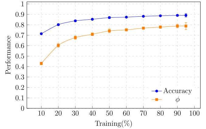
FIG. 19. Training and validating five classes: ['A, ' 4] , ['D, ' 4] , ['A, ' 6] , ['D, ' 6] and ['E, ' 6] . We generate (52 + 50 + 76 + 77 + 77) matrices. There are 6699 1's and 6711 0's. The method is NB.
