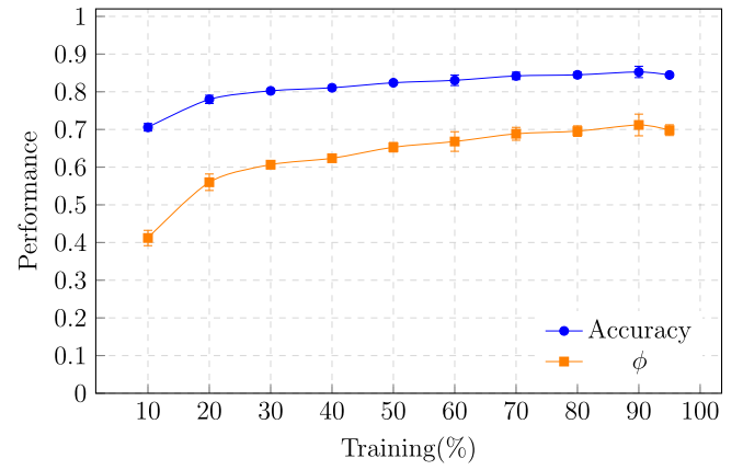
FIG. 18. Training and validating four classes: ['A, ' 4] , ['D, ' 4] , ['A, ' (3,1),1] , and ['A, ' (2,2),1] . We generate (52 + 50 + 70 + 54) matrices. There are 5503 1's and 5512 0's. The method is NB.
