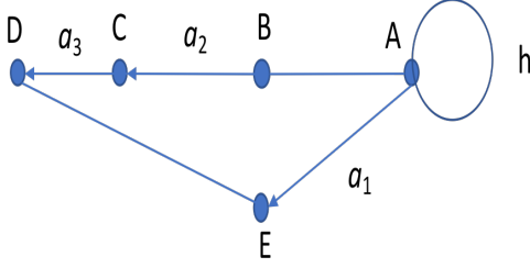
Fig. 3: A counter-example to Proposition 2 for the case of open and irreversible ZC-GBTS.
