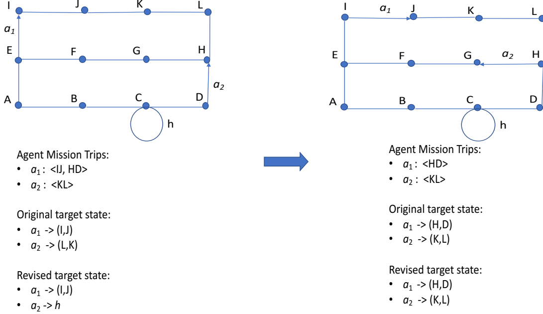
Fig. 7: A partial execution of the algorithm of Figure 6 on the example transport system that was introduced at the beginning of Section V.
