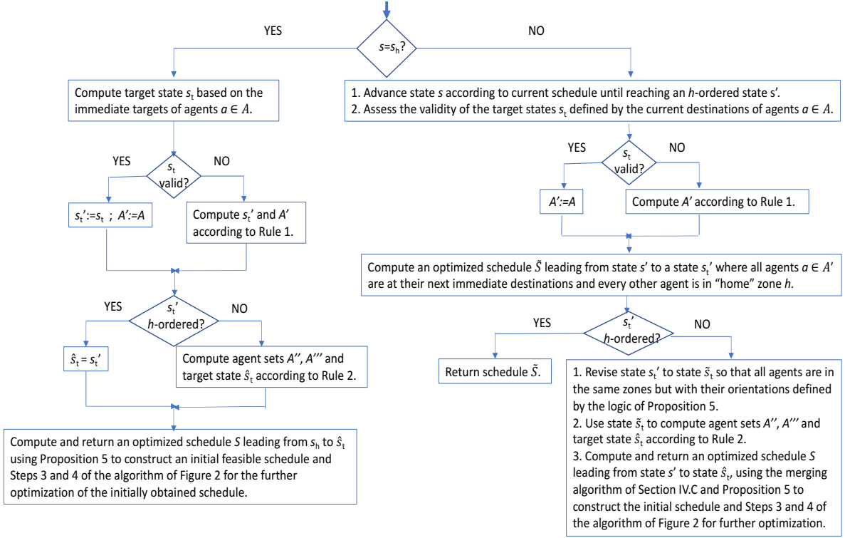
Fig. 6: A flowchart representing the adaptation of the heuristic algorithm of [4] for the generation and solution of the subproblems to be addressed by the MPC framework for open and irreversible ZC-GBTS that is developed in this work.
