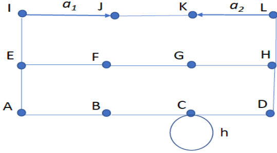
Fig. 5: The final state s' of the guidopath-based transport system considered in the first part of the example of Section V.
