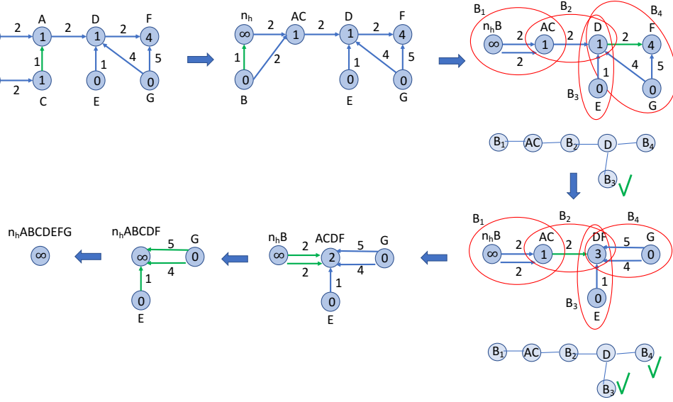
Figure 8: The DAGs generated and processed by Algorithm 6 in Example 51.
