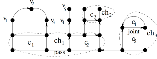
(a) A PDG \hat{G}(s) and the "chain" structure that is recognized in it.
