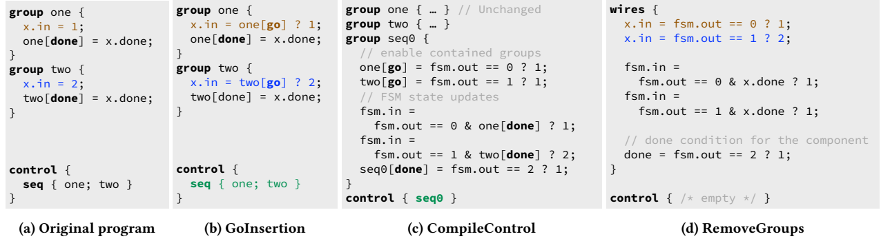
Figure 2: Calyx realizes the execution schedule by encoding it with structural components. After the COMPILECONTROL pass (c), the fsm register encodes the current state for the seq statement.
