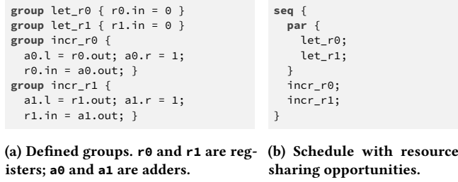
Figure 3: Resource sharing example. Since incr_r0 and incr_r1 do not run in parallel, they can share their adders.
