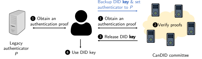
(b) Key backup and recovery workflow.
