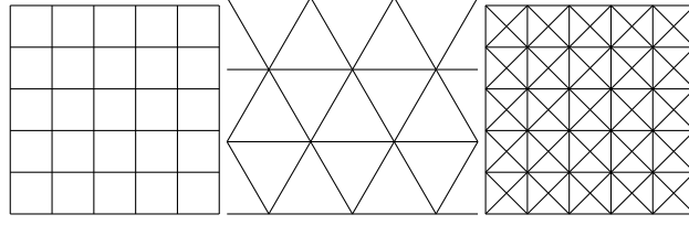
FIG 2. The square, triangular and tetrakis square lattices are examples of tilings with reflecting families of lines such that the quotient by the reflection group is a bounded convex region of the plane.
