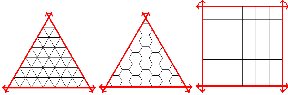
FIG 3. The triangular, hex and square lattice configurations with open boundary condition.
