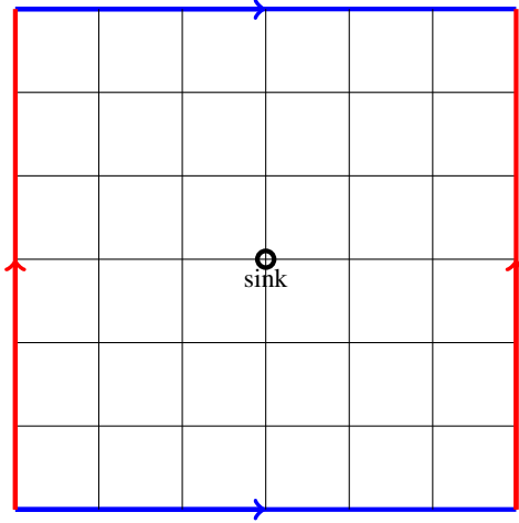
FIG 1. The square lattice configuration with periodic boundary condition and a single sink.
