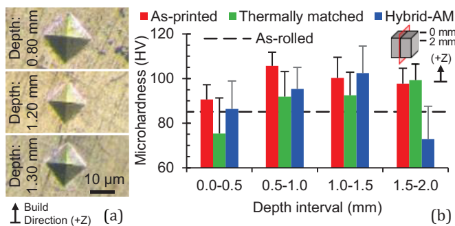
Fig. 5. (a) Representative Vicker's indents and (b) regional microhardness at various depths in printed WE43.
