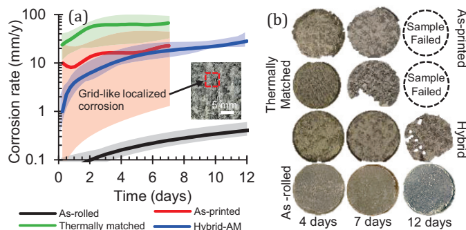
Fig. 8. (a) Corrosion rate and (b) dissolution WE43 disc.
