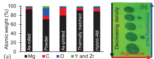
Fig. 7. (a) Energy dispersive X-ray spectroscopy of printed WE43 discs and (b) soot in print chamber.
