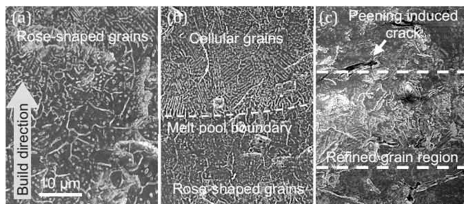
Fig. 4. Representative microstructure of (a) as-printed and (b) thermally matched, and (c) refined grains in Hybrid-AM WE43 at 1.2 mm depth.
