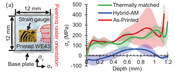
Fig. 6. (a) Strain gage to measure (b) residual stress in printed WE43.
