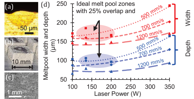
Fig. 2. PBF of WE43: (a) single-track melt pool, (b) cuboid, (c) CT scan of high density cross section printed with 32.1 \text{J}/\text{mm}^3 , and (d) single-track process map optimizing melt pool dimensions.
