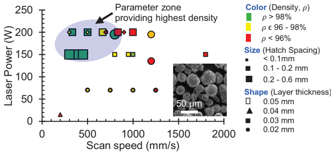
Fig. 1. PBF process parameter map for Mg alloys. Modified from [9].
