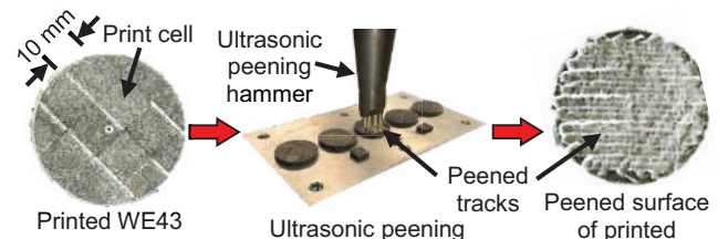
Fig. 3. Inter-layer ultrasonic peening during PBF.
